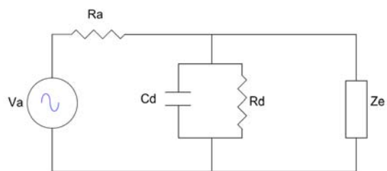
Figure 2: Equivalent circuit of a solar rectenna.
