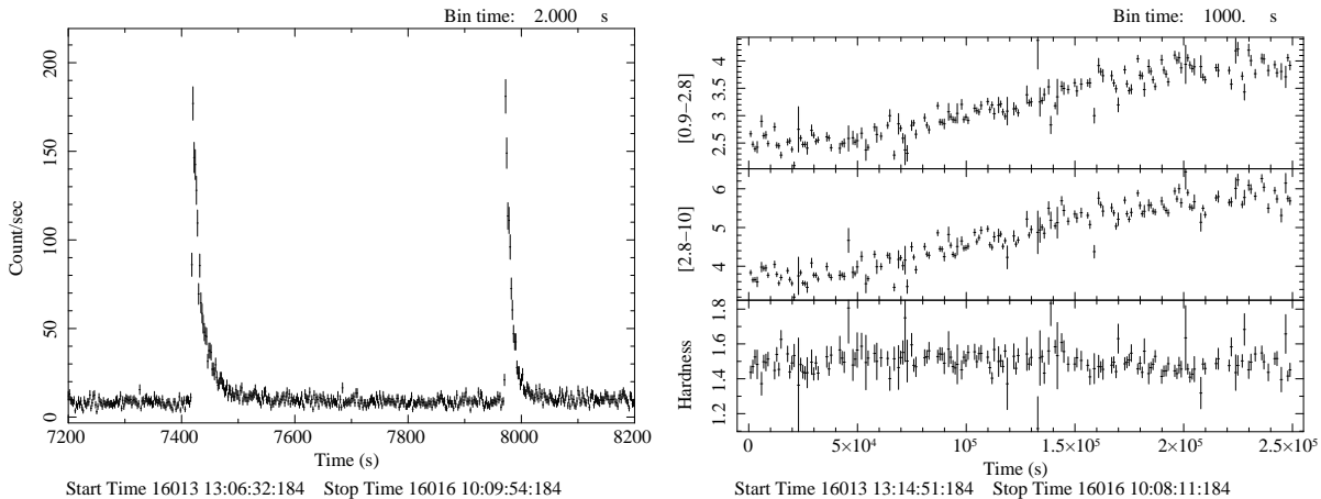
Figure 1. Left: Suzaku XIS0 light curve in the energy range 0.9 - 10 keV showing two of the nine type-I bursts which occurred during the 250-ks observation. Right: Suzaku XIS0 light curves in the energy range 0.9 - 2.8 keV (top panel), 2.8 - 10 keV (middle panel), and the corresponding hardness ratio (bottom panel).
