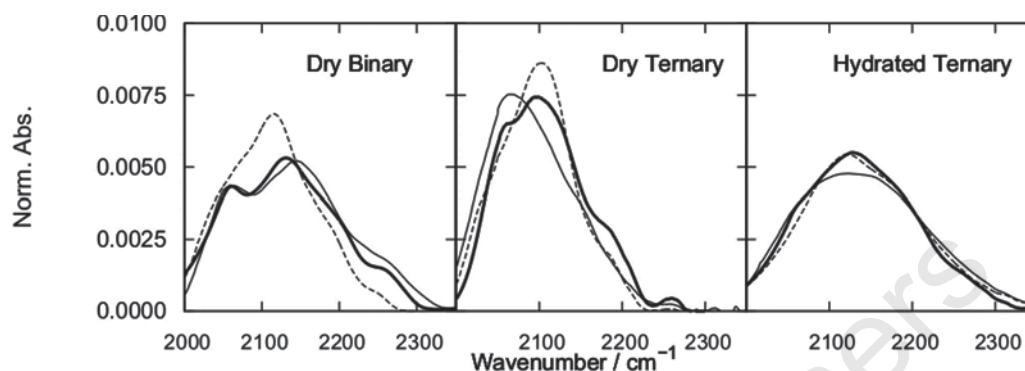
Fig. (3). Normalized spectra of the Water Association Band (WAB) at 300 K. Thick lines: trehalose [145]; dashed lines: sucrose [146,168]; thin lines: maltose [54]. Reproduced from Eur.Phys.J.E , 36, 2013, 79, Proteins in amorphous saccharide matrices: structural and dynamical insights on bioprotection , Giuffrida, S.; Cottone, G.; Bellavia, G.; Cordone, L. [148] with kind permission of The European Physical Journal (EPJ).
