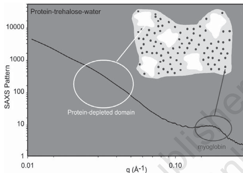
Fig. (6). A typical SAXS pattern for a trehalose-myoglobin-water dry sample. The protein and the protein-poor domains signals are highlighted. Sample features are pictorially sketched in the upper right region inside the plot: the protein poor domains are in white; proteins in black. Reproduced from Ref. [168] with permission from the PCCP Owner Societies.
