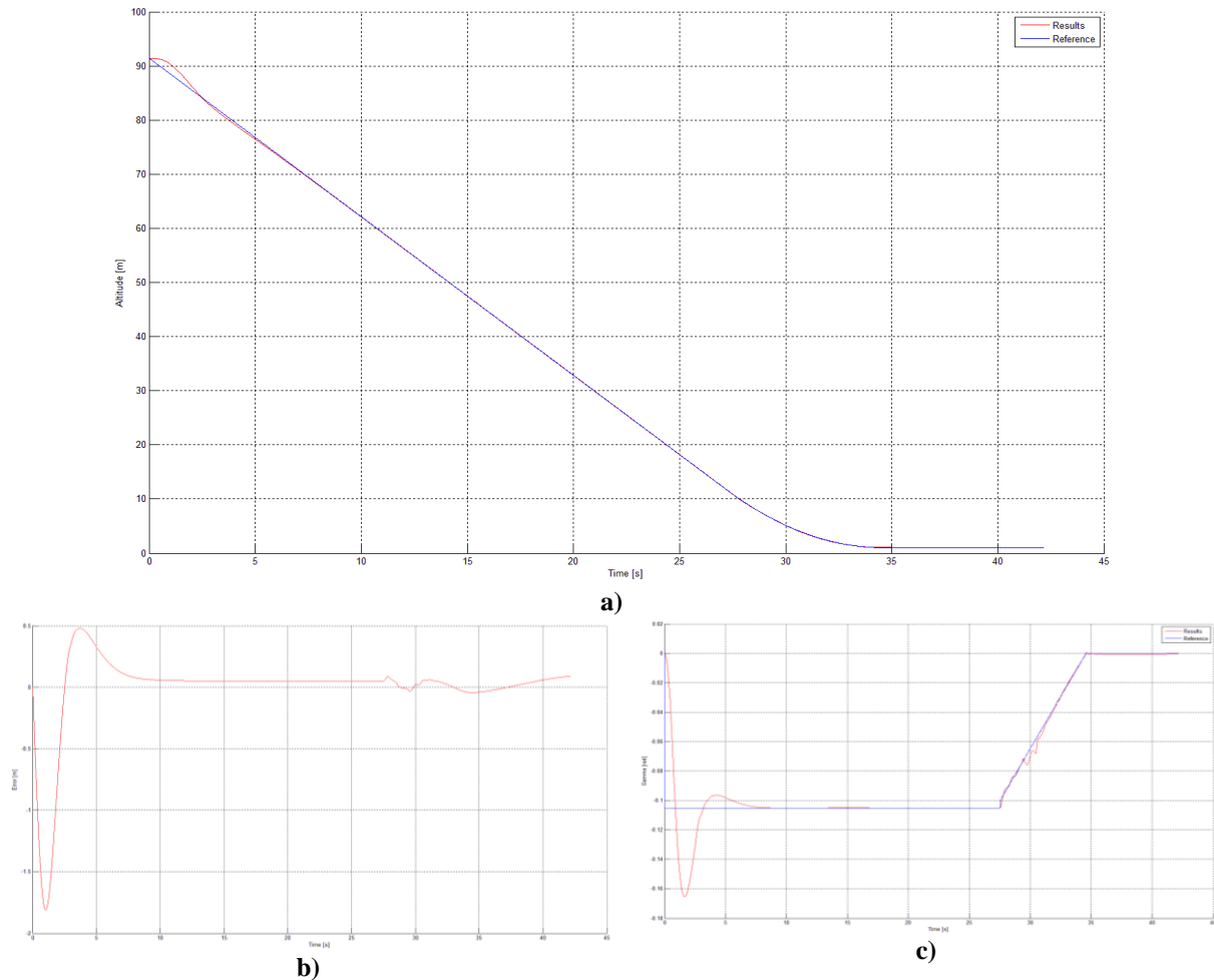
Fig. 2 Indirect flight path following:
