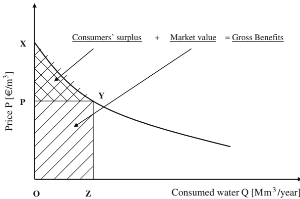
Fig. 2 Demand function for water and components of benefits
