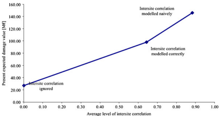
Fig. 6 Present expected damage in the BAU case as a function of the average level of intersite correlation among supply sources
