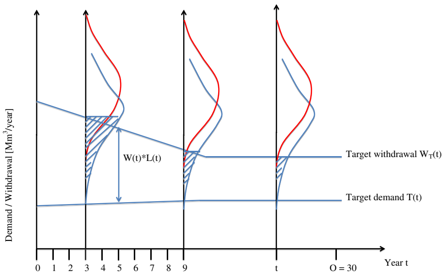
Fig. 1 Schematic of the risk assessment procedure
