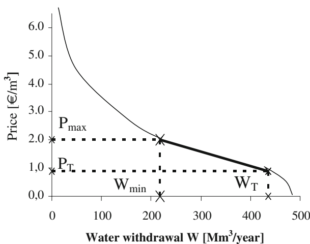
Fig. 3 Linear specification of the price – demand relationship of municipal water: amounts supplied less than W_{min} are considered outside the range of applicability of the linear relationship
