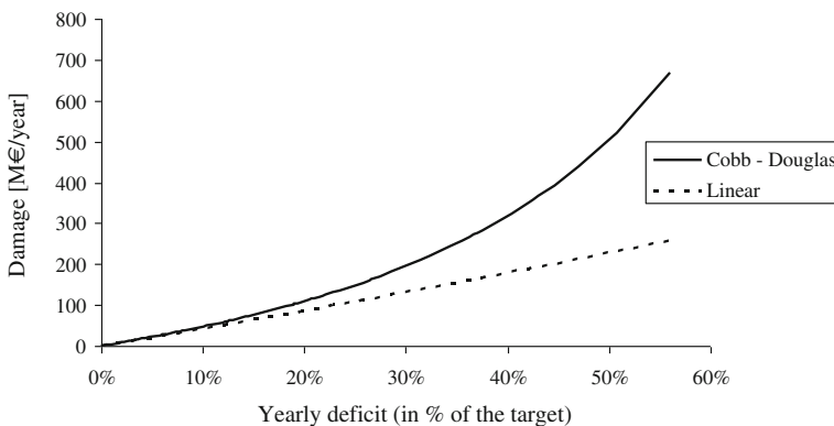
Fig. 4 Comparison of damage – deficit relationships obtained from a log-linear (Cobb-Douglas) and from a linear demand function for municipal water. Deficit is expressed in percentage of the yearly target demand
