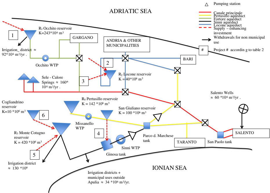
Fig. 5 Schematic representation of the water resources system supplying municipal uses in Apulia. The numbers inside the boxes refer to supply-enhancing projects # (see Table 2)
