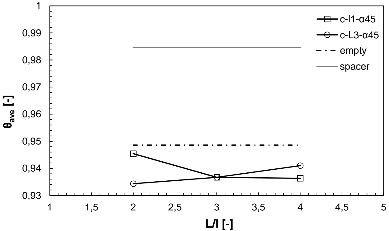
Figure 18. Average polarization factor \theta_{ave} as a function of the profile pitch-to-size ratio for c-\alpha45 channels at Re = 8 . Empty and spacer-filled channels are also reported for comparison.
