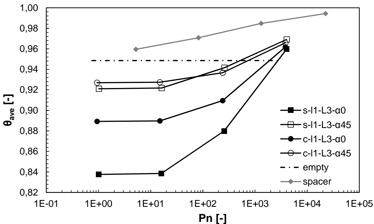
Figure 13. Average polarization factor \theta_{ave} as a function of the dimensionless power number for l1-L3 , empty and spacer-filled channels.
