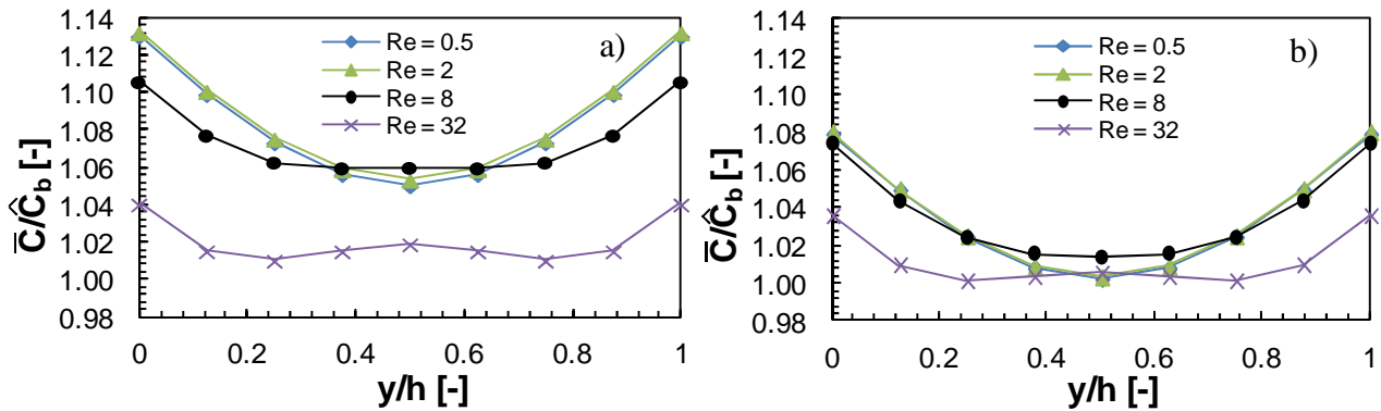
Figure 9. Normalized area-averaged electrolyte concentration in the direction perpendicular to the membrane-solution interfaces at various Re for channels (a) c-11-L3- \alpha 0 and (b) c-11-L3- \alpha 45 .
