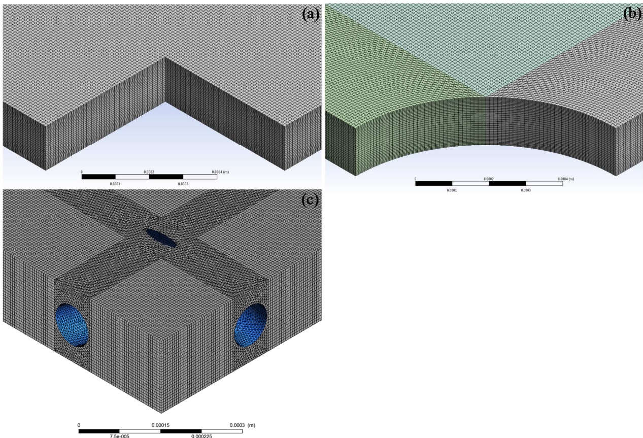
Figure 5. Discretization of the Unit Cell for (a) s-II-L3 channel, (b) c-II-L3 channel and (c) spacer-filled channel.
