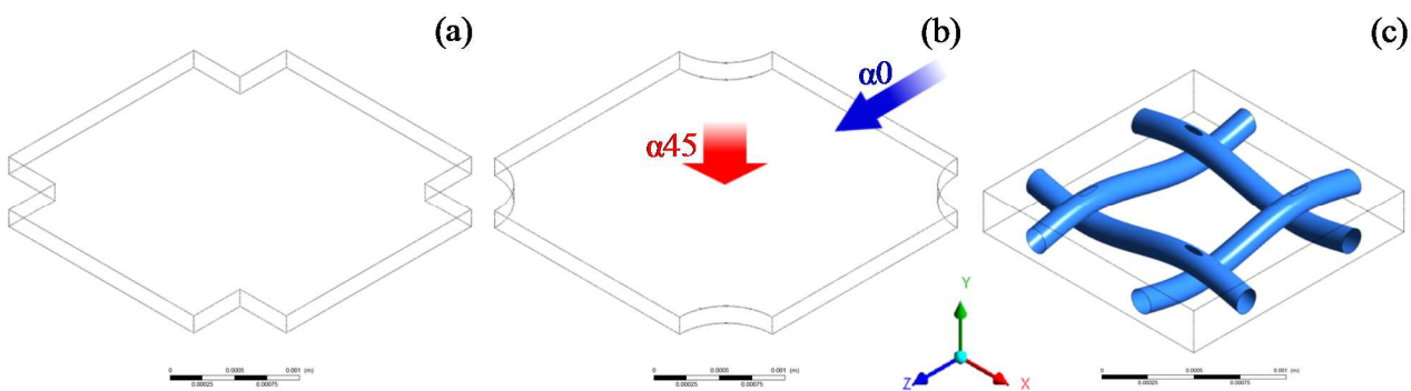
Figure 4. Unit Cell geometry for (a) s-II-L3 channel, (b) c-II-L3 channel and (c) spacer-filled channel.
