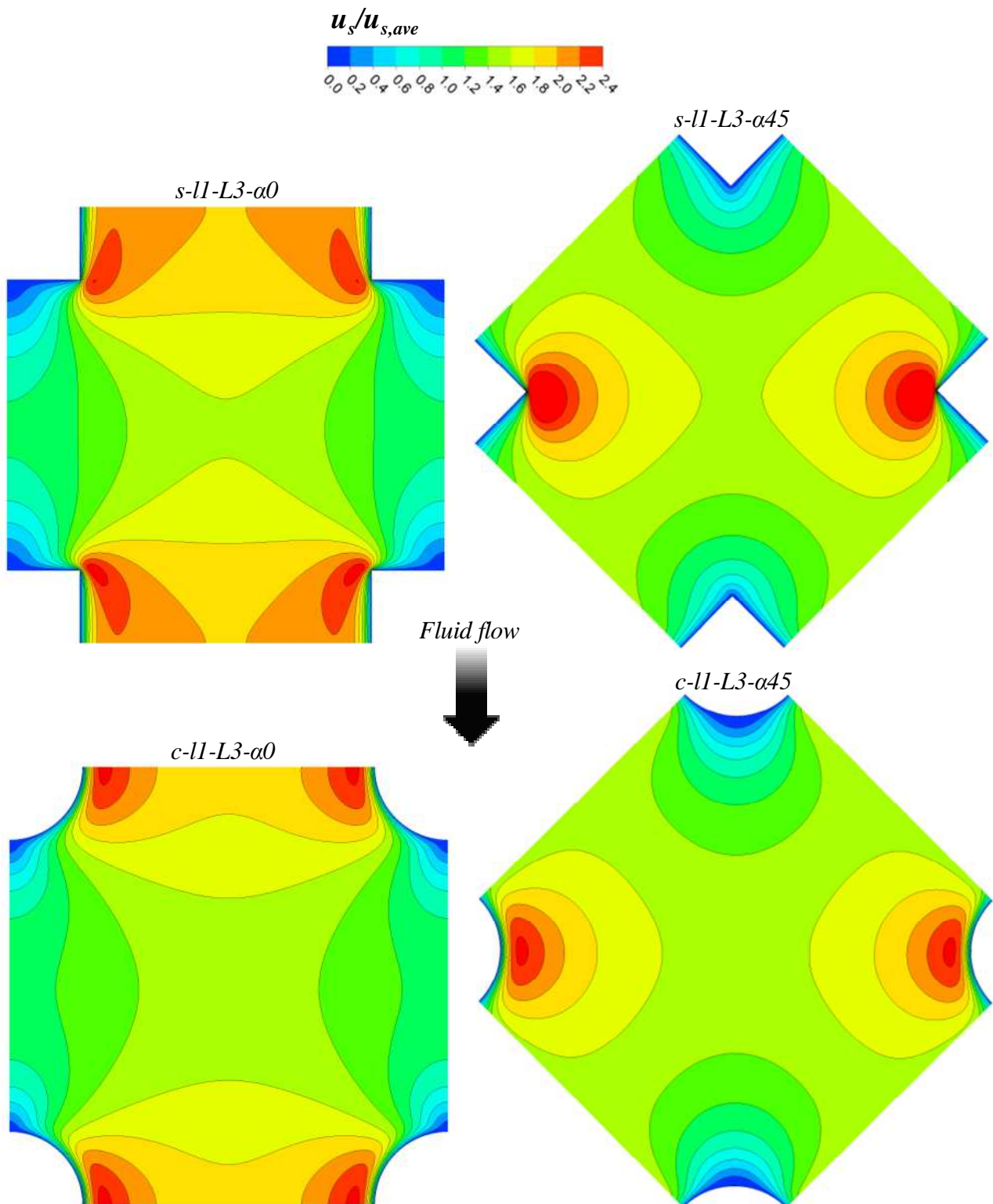
Figure 6. Maps of the normalized streamwise velocity component on the x - z midplane for s -11- L3 - \alpha0 , s -11- L3 - \alpha45 , c -11- L3 - \alpha0 and c -11- L3 - \alpha45 channels at Re = 8 .
