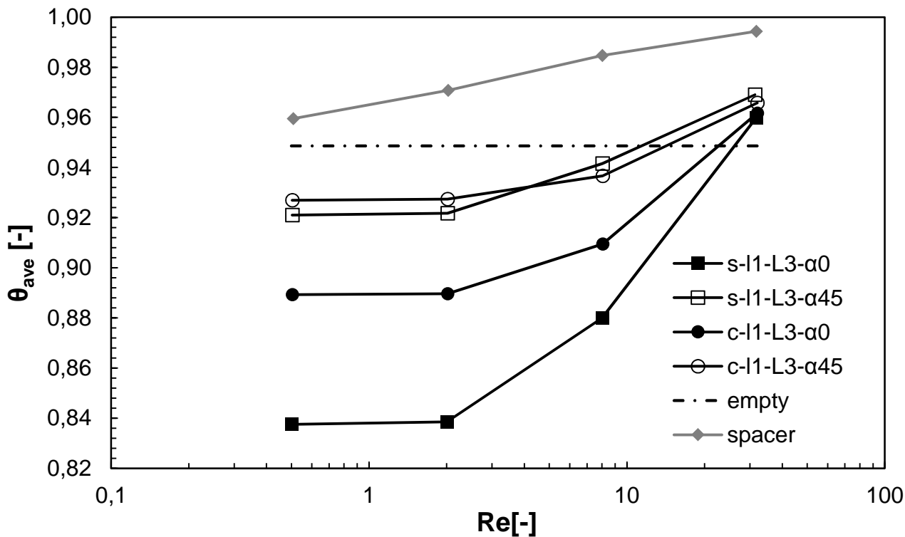
Figure 12. Average polarization factor \theta_{ave} as a function of the Reynolds number for l1-L3 , empty and spacer-filled channels.
