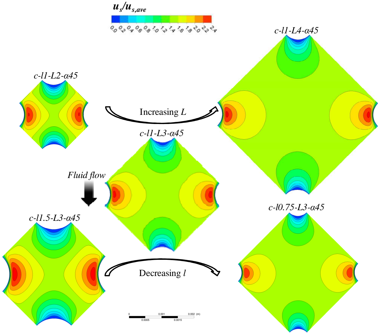
Figure 14. Maps of the normalized streamwise velocity component on the x - z midplane for c -11-L2- \alpha 45, c -11-L4- \alpha 45, 11-L3- \alpha 45, 11.5-L3- \alpha 45 and 10.75-L3- \alpha 45 channels at Re = 8 .
