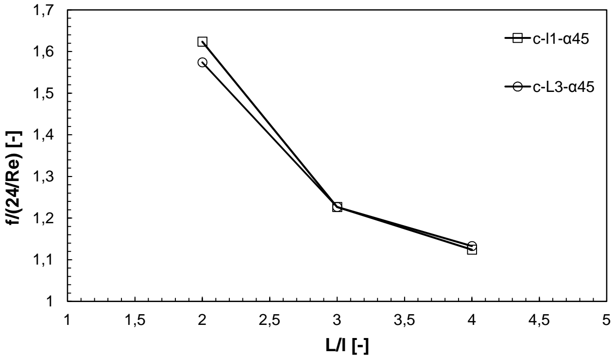
Figure 17. Fanning friction factor normalized by that pertaining to an empty channel ( 24/Re ) as a function of the profile pitch-to-size ratio for c-\alpha45 channels at Re = 8 .
