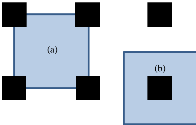
Figure 3. Possible equivalent Unit Cells. Type (a) was chosen in the present work.
