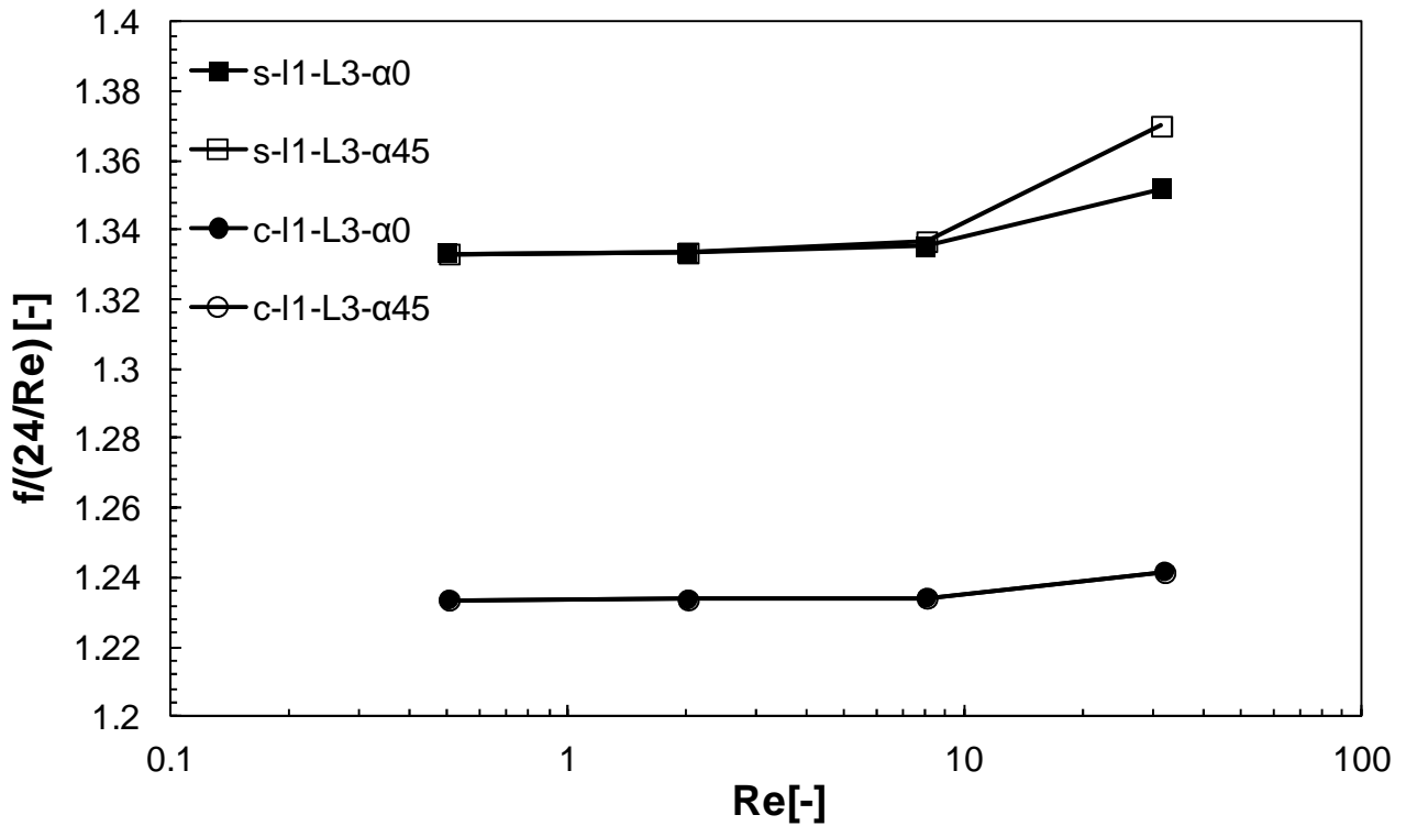
Figure 10. Fanning friction factor normalized by that pertaining to an empty channel ( 24/Re ) as a function of the Reynolds number for l1-L3 profile configurations.
