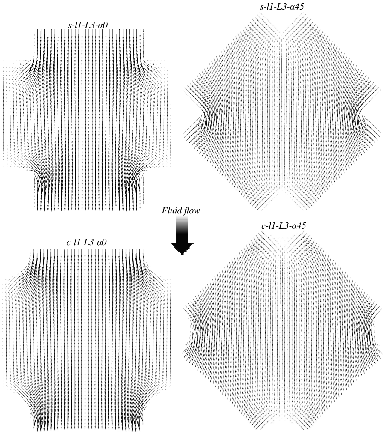
Figure 7. Velocity vector plots on the x - z midplane for s-II-L3-\alpha0 , s-II-L3-\alpha45 , c-II-L3-\alpha0 and c-II-L3-\alpha45 channels at Re = 8 .
