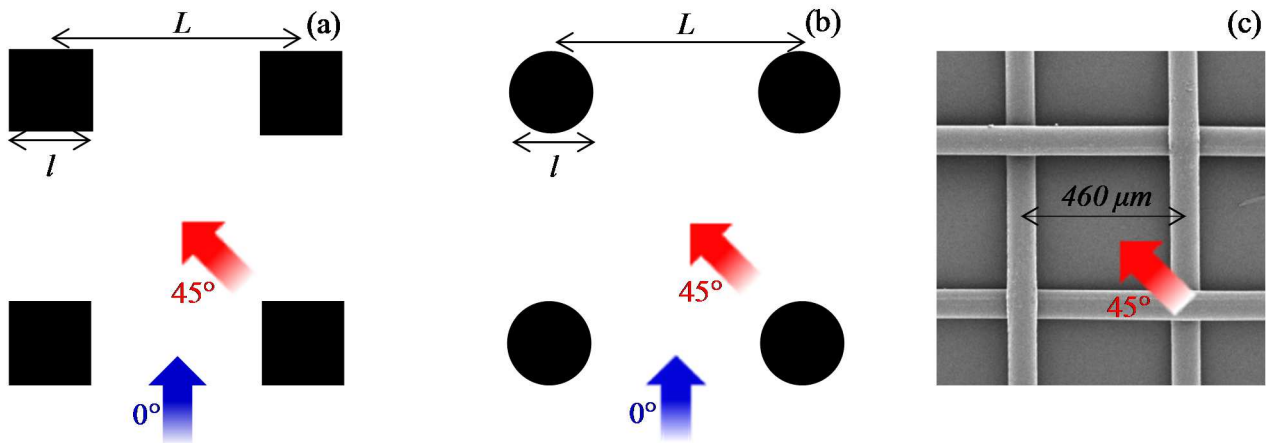
Figure 2. Sketches of the two profile geometries simulated (a-b). The woven wire spacer is also shown for comparison (c).
