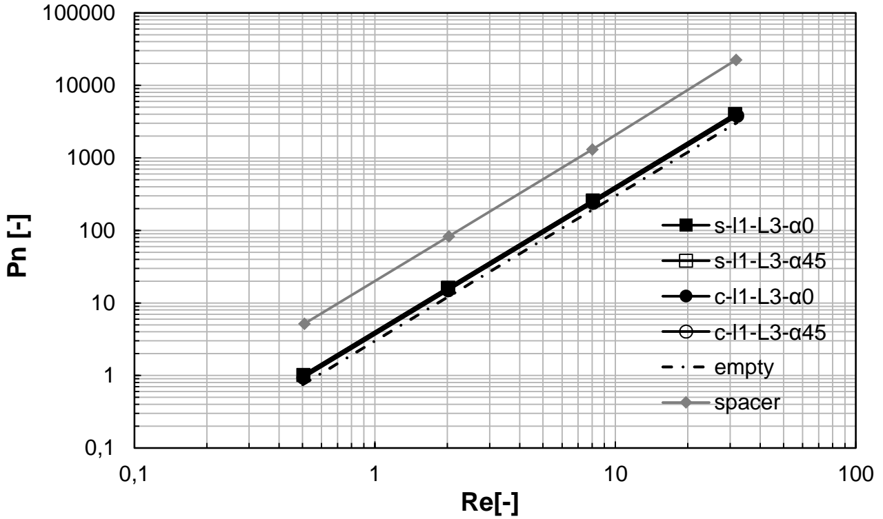
Figure 11. Dimensionless power number as a function of Reynolds number for l1-L3 , empty and spacer-filled channels.
