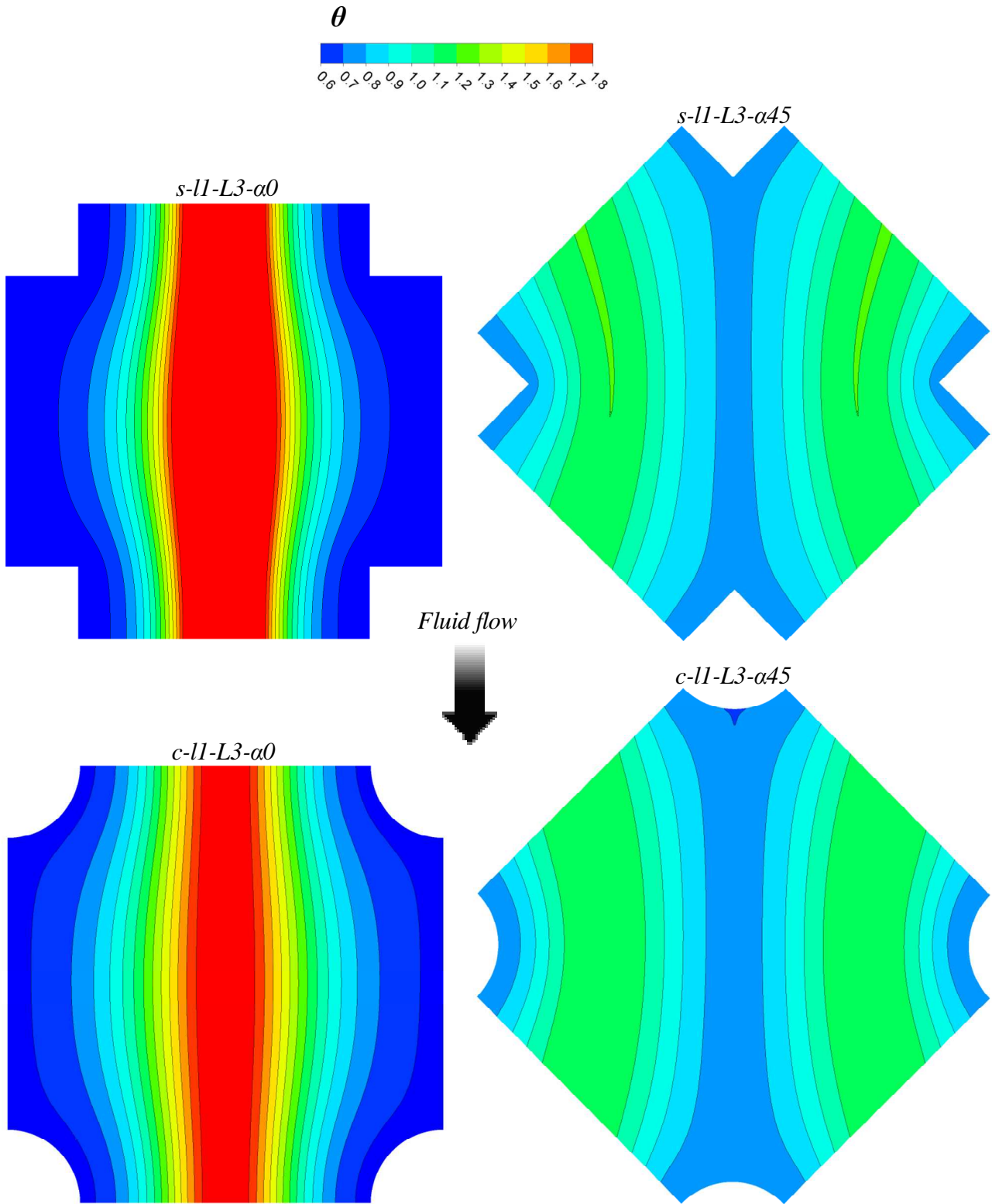
Figure 8. Maps of the local polarization factor \theta = \hat{C}_b / C_w on one of the fluid-membrane interfaces for s-11-L3- \alpha 0 , s-11-L3- \alpha 45 , c-11-L3- \alpha 0 and c-11-L3- \alpha 45 channels at Re = 8 .
