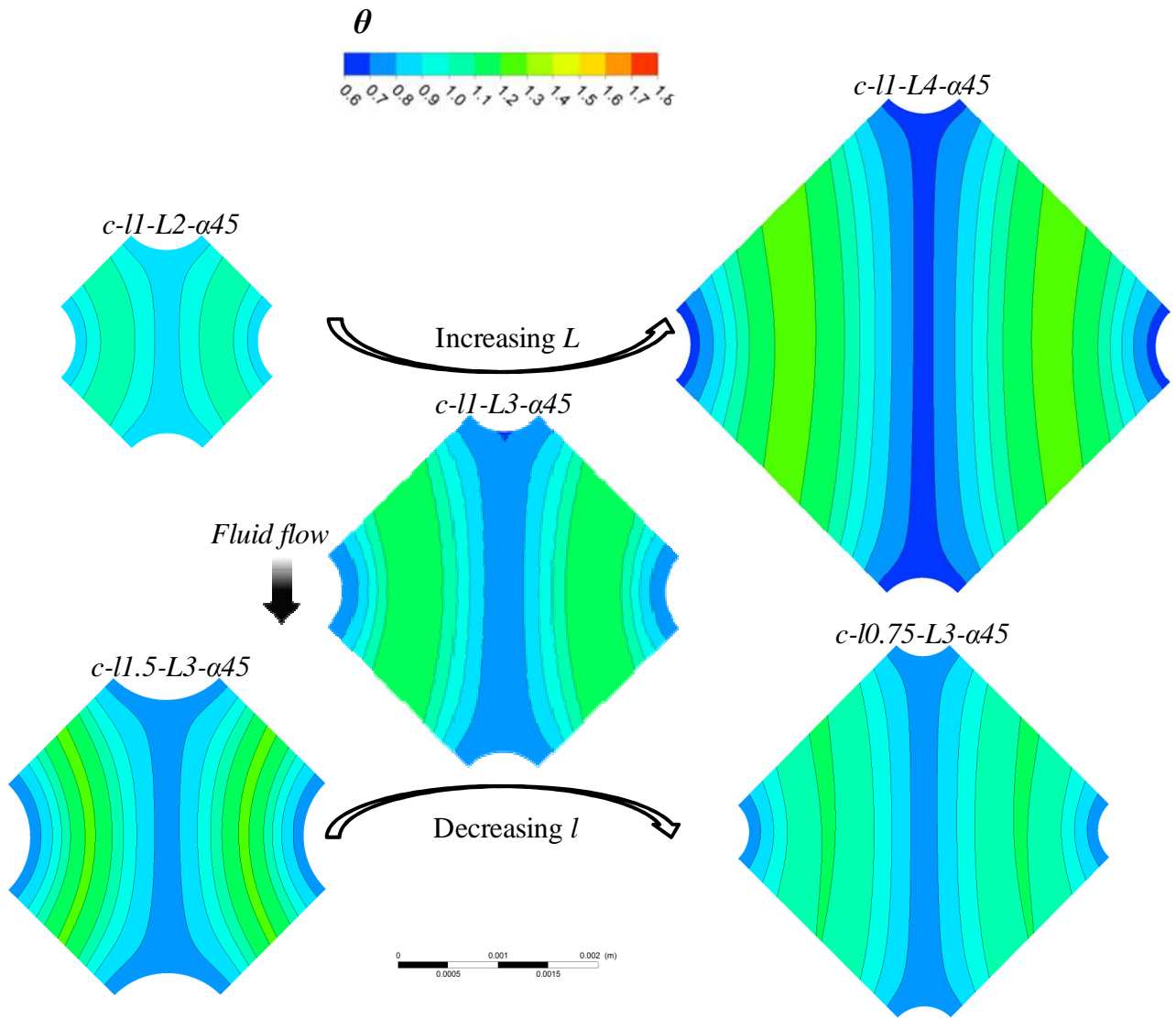
Figure 16. Maps of the local polarization factor \theta = \hat{C}_b / C_w on one of the fluid-membrane interfaces for c-11-L2-\alpha45 , c-11-L4-\alpha45 , 11-L3-\alpha45 , 11.5-L3-\alpha45 and 10.75-L3-\alpha45 channels at Re = 8 .
