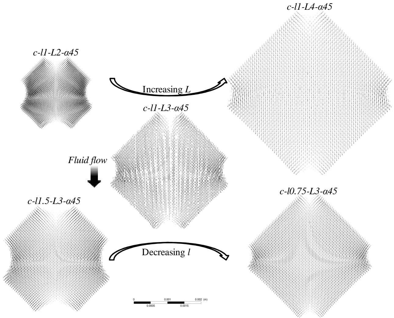
Figure 15. Velocity vector plots on the x - z midplane for c-11-L2-\alpha45 , c-11-L4-\alpha45 , 11-L3-\alpha45 , 11.5-L3-\alpha45 and 10.75-L3-\alpha45 channels at Re = 8 .
