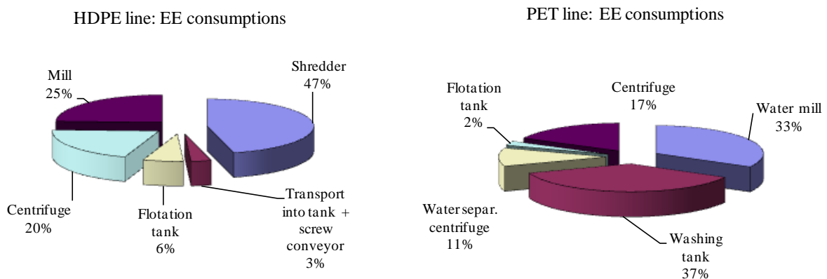
Figure 5. Electrical energy use distribution for the two “wet” separation lines of HDPE and PET.
