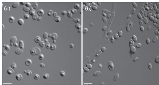
Fig. 3. Micrographs of growth of strain U88A2 T . (a) Vegetative cells after 3 days at 25 °C on 5% malt extract agar; (b) pseudohyphae after 15 days at 25 °C on Dalmat plates. Bars, 10 μm.
