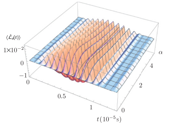
FIG. 2. (Color online) Mean value of \hat{\mathcal{L}}_x(t) for a cantilever in the initial state as given by Eq. (10) with C_0 = C_1/\alpha = 1/\sqrt{1+\alpha^2} and C_n = 0 otherwise. The BEC consists of N = 10^{387} Rb atoms and \langle \hat{\mathcal{L}}_{x,y}(0) \rangle = 0 , \langle \hat{\mathcal{L}}_z(0) \rangle = 100 . We have used B_z^0 = 3 \times 10^{-6} mT and G_c \approx 1.8 \times 10^3 \mu\text{T}/\mu\text{m} .
