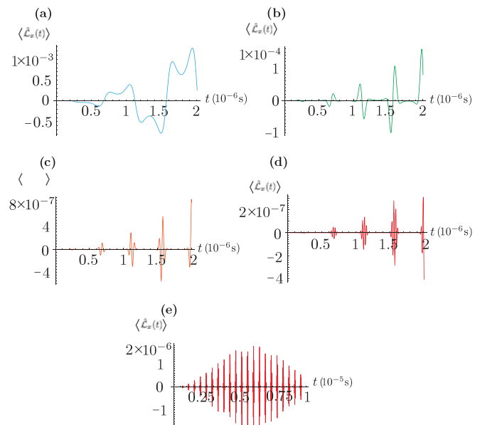
FIG. 4. (Color online) Time evolution of \langle \hat{\mathcal{L}}_x(t) \rangle for a coherent initial state of the cantilever with (a) |\alpha|^2 = 1 , (b) 5, (c) 15, and (d) 20. For the same parameter as in (d), the plot (e) shows that the carrier frequency \omega_L is not significantly affected.
