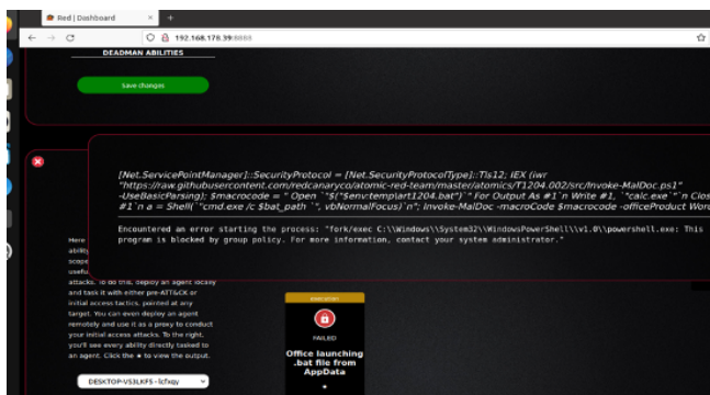
Figure 9. APT29/41-v1 Execution – Denied
