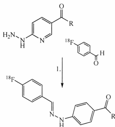
Scheme 1.8 Scheme to show the chemoselective radiofluorination reaction via hydrazone bond formation between HYNIC or a HYNIC-functionalised peptide and [ ^{18}\text{F} ]FB-CHO. (1) MeCN/ \text{KH}_2\text{PO}_4 buffer, \Delta\text{T} , 10 min. R = OH, -Tyr 3 -Thr 8 -octreotide, -Tyr 3 -Thr 8 (NH 2 )-octreotide, -substance-P (Bruus-Jensen et al. 2006)
