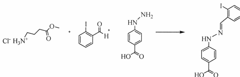
Scheme 2.10
