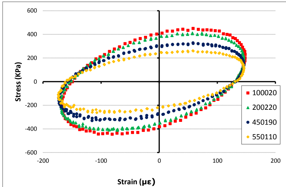
Figure 8 Evolution of hysteresis loop during a fatigue test
