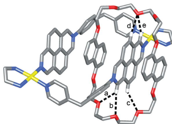
Fig. 5 Stick representation of the solid state structure of catenane 1a(7) · 6\text{PF}_6 showing [C–H...O] hydrogen bonds. [H...O] and [C...O] distances and [C–H...O] angles: a 2.71, 3.40 Å, 130°; b 2.68, 3.61 Å, 167°; c 2.77, 3.52 Å, 135°; d 2.39, 3.28 Å, 156°; e 2.79, 3.59 Å, 143°. Solvent molecules, counterions and remaining hydrogen atoms are omitted for clarity. Colour scheme: C, grey; O, red; N, blue; H, white; Pd, yellow.
