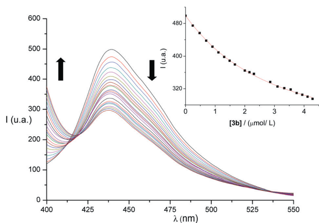
Fig. 3 Fluorescence spectra ( \text{H}_2\text{O} , 293 K, \lambda_{\text{exc}} = 326 \text{ nm} ) of a solution of 1b · 6\text{NO}_3 ( 1.0 \times 10^{-6} \text{ M} ) after successive addition of aliquots of a solution of guest 3b ( 1.0 \times 10^{-5} \text{ M} ) and host 1b · 6\text{NO}_3 ( 1.0 \times 10^{-6} \text{ M} ). Inset: emission intensity at \lambda_{\text{max}} = 439 \text{ nm} vs. concentration of 3b fitted to a 1 : 1 isotherm.
