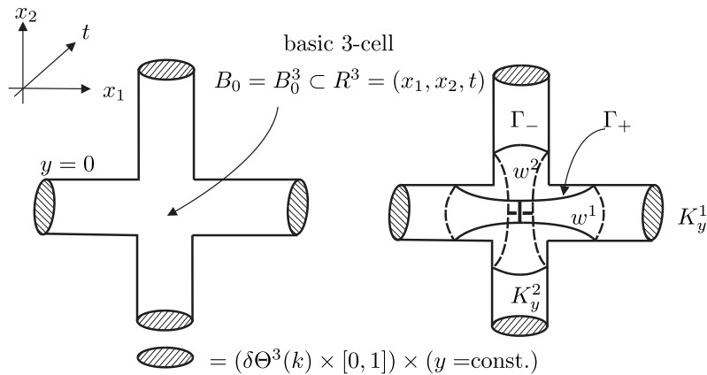
Fig. 6. In the right hand side we see K_y = K_y^1 + K_y^2 which is obtained by deleting the region intermediary between \Delta_\pm (= the disks cobounding \Gamma_\pm ) and then letting each K_y^\epsilon become thin along the waist w^\epsilon .
