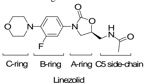
Figure 1. Structure and portions nomenclature of Linezolid
