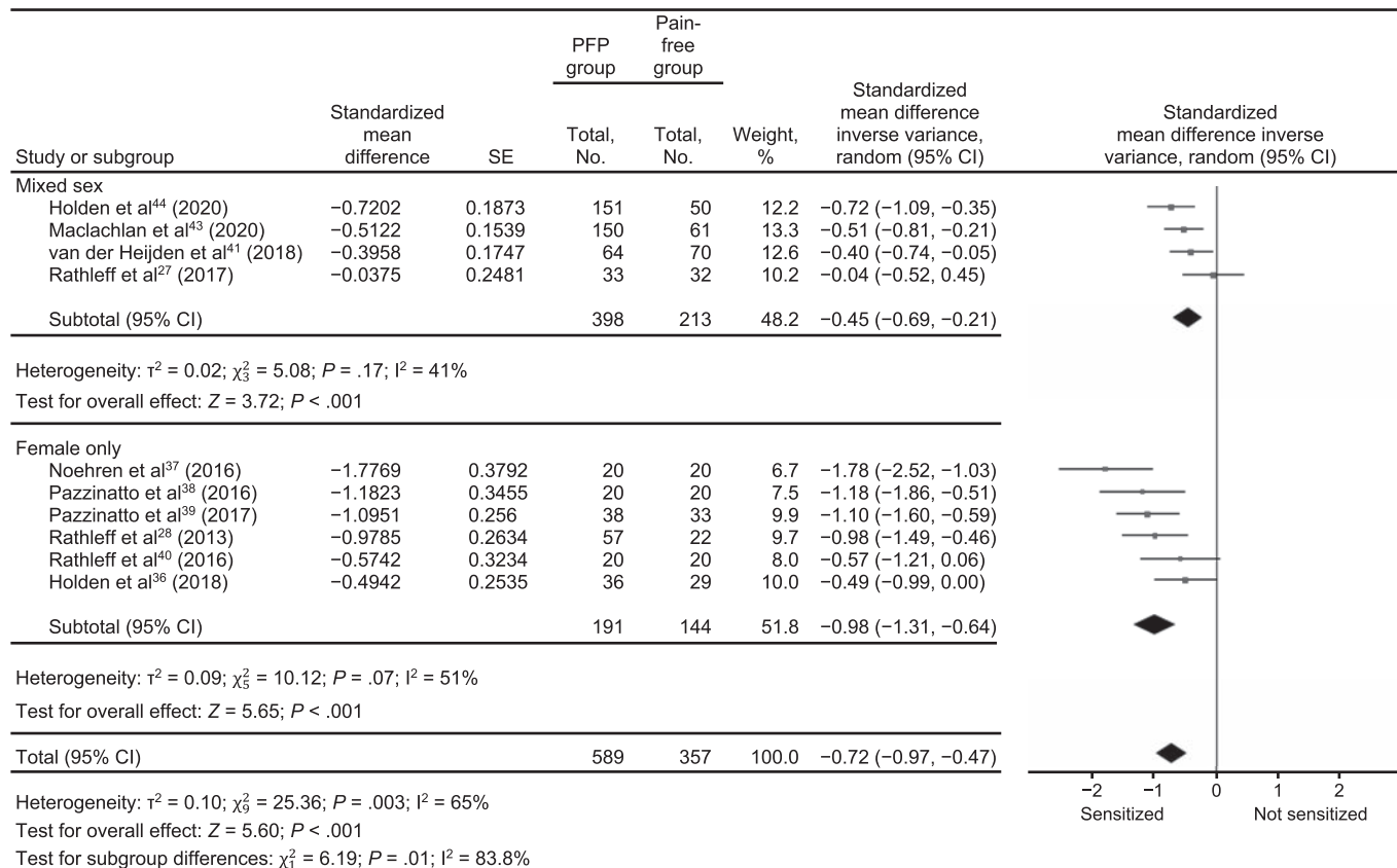
Figure 3. Meta-analysis results of remote pressure pain thresholds. a Abbreviation: PFP, patellofemoral pain.
