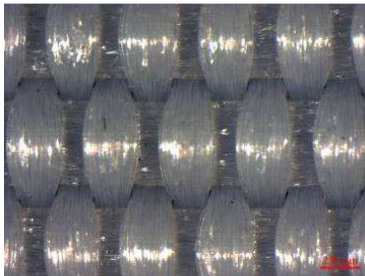
Figure 8: 40x magnification optical microscope images of tested specimen in weft direction (cyclic test 2).
