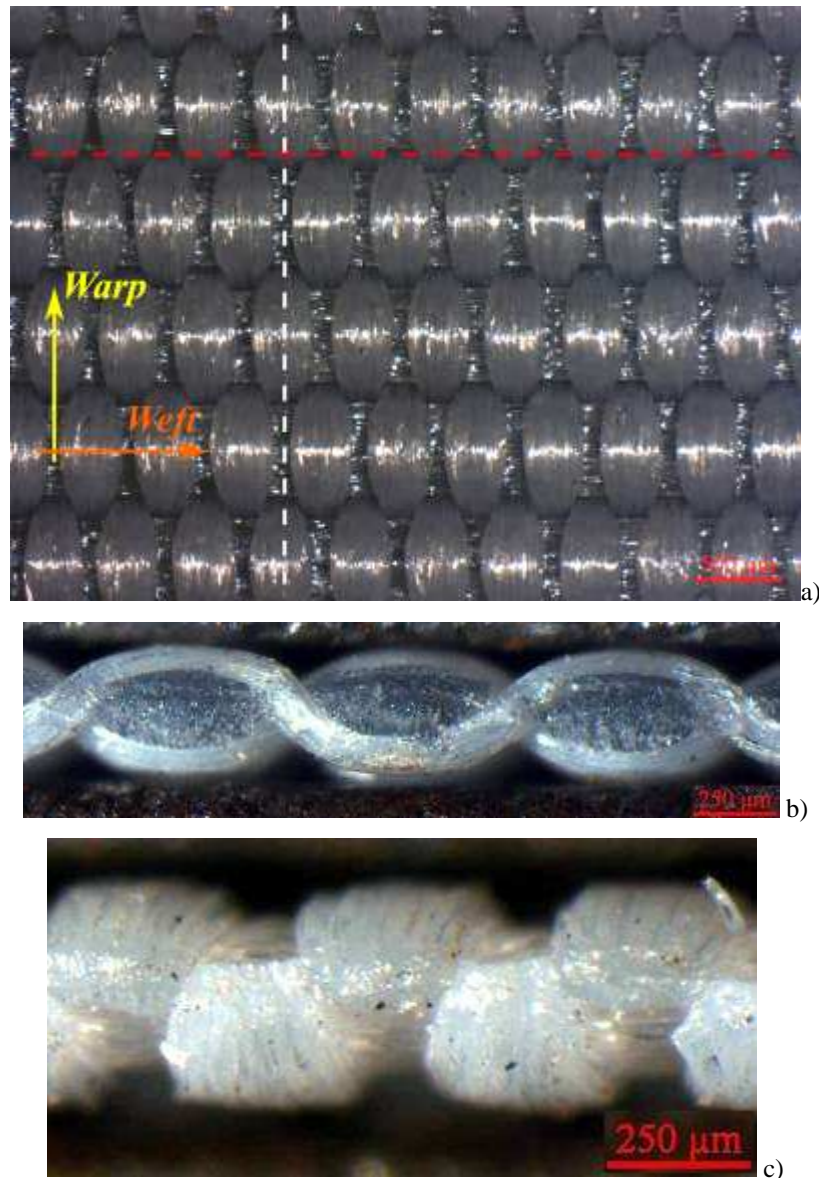
Figure 1: Microscope photos of the specimen - a) 20x particular of the specimen. b) 40x particular of the cross-section in the weft direction. c) 40x particular of the cross-section in the warp direction.
