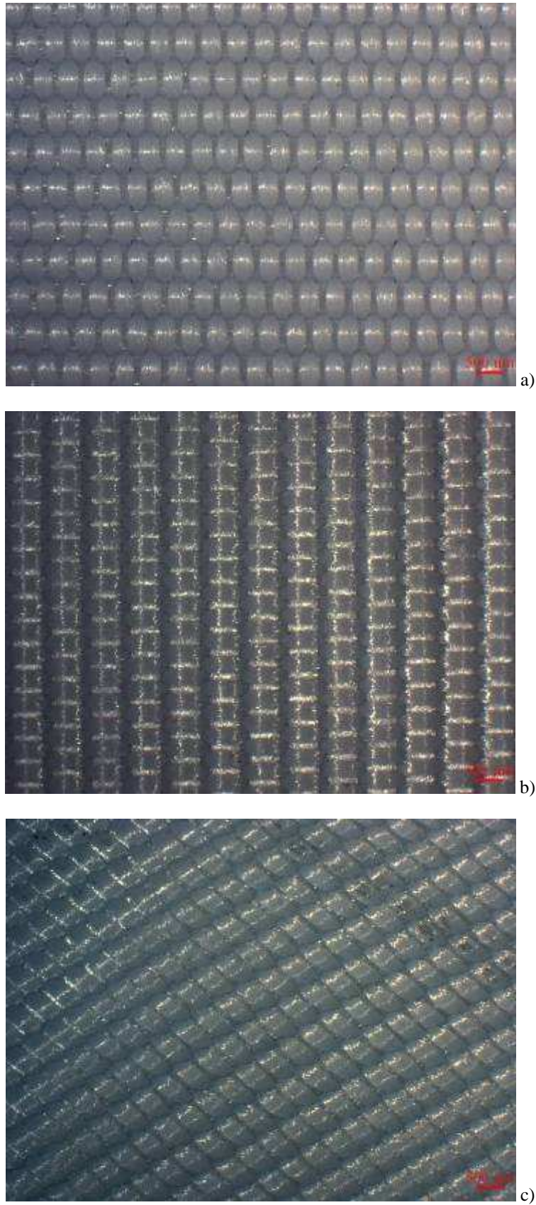
Figure 6: Optical microscope images of tested specimens (10x magnification): a) Weft direction; b) Warp direction; c) Bias direction.
