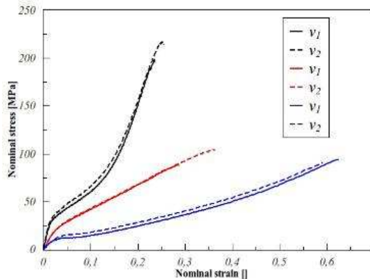
Figure 3: Tensile test results: (black lines) weft direction; (red lines) warp direction. (blue lines) bias direction.
