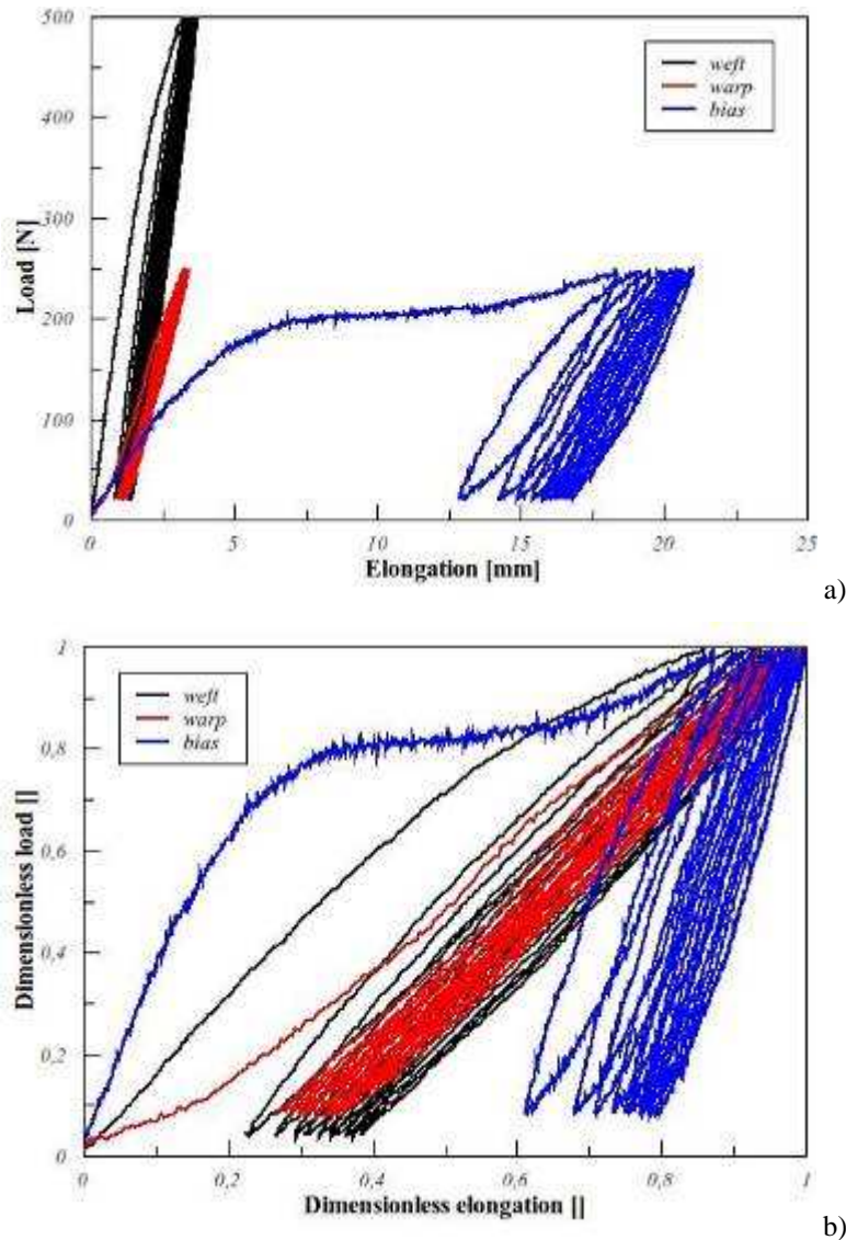
Figure 5: Cyclic test 2 results: a) Load vs elongation; b) Dimensionless load vs dimensionless elongation.
