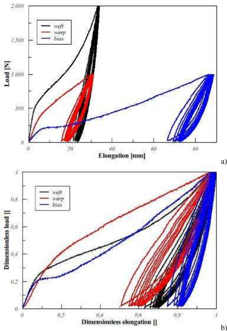
Figure 4: Cyclic test 1 results: a) Load vs elongation; b) Dimensionless load vs dimensionless elongation.
