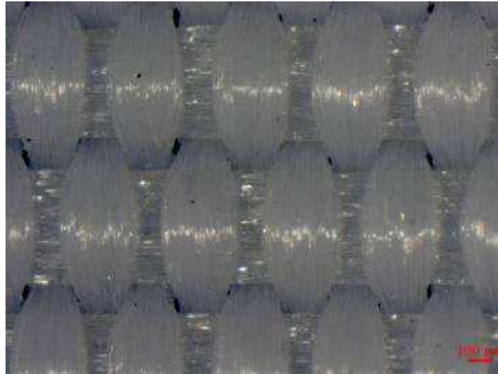
Figure 7: 40x magnification optical microscope images of tested specimen in weft direction (tensile test).
