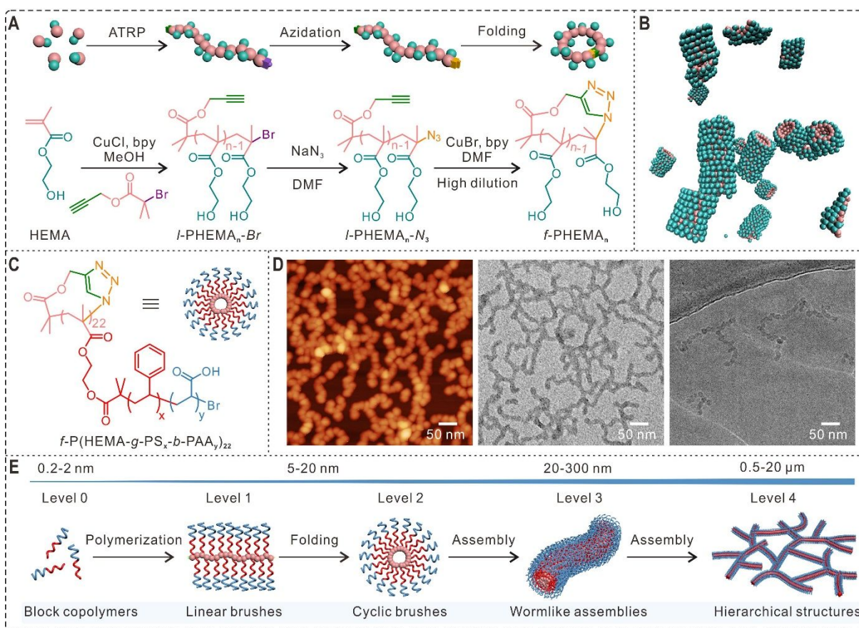
Fig. 4 Hierarchical nanostructures self-assembled from cyclic polymers. (A) Scheme of the synthesis of I -PHEMA _n -Br and its azidation and folding into the cyclic topology. (B) Molecular dynamic simulation snapshot showing the self-assembly of f -PHEMA _{15} into wormlike structures. (C) Molecular structure and scheme of cyclic brush polymer f -P(HEMA- g -PS _x - b -PAA _y ) _{22} . (D) AFM (left), TEM (middle), and cryo-TEM (right) images showing the self-assembly of cyclic brush polymers into 1D wormlike assemblies and hierarchical structures at 0.4 mg mL ^{-1} in water. (E) Schematic of the formation of hierarchical structures by synthetic polymers via biomimetic folding and self-assembly. Copyright 2021 The Authors. Reproduced with permission. 32 Published by Springer Nature.
