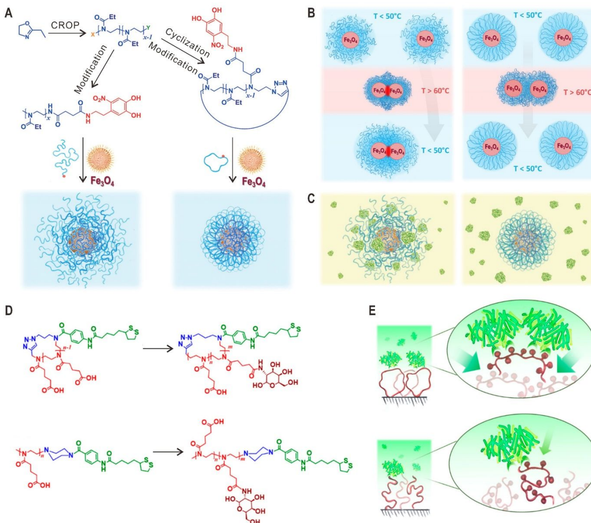
Fig. 6 Cyclic polymers for surface functionalization. (A) Synthesis of linear and cyclic PEOXAs by cationic ring opening polymerization (CROP) and post-modification for the surface functionalization of Fe 3 O 4 NPs. (B) Temperature-induced transitions for suspensions of NPs coated with linear (left) and cyclic (right) PEOXAs. (C) Schematics showing the interaction of BSA with linear (left) and cyclic (right) PEOXA brush-coated NPs. (D) Synthesis of cyclic and linear glycopolymers by introducing galactose moieties into to corresponding PCPOXA chains. (E) Functional surfaces modified with cyclic glycopolymers reveal more efficient presentation of functional groups and increased lectin-binding ability. Copyright 2017. Reproduced with permission from John Wiley and Sons Inc. 100 Copyright 2020. Reproduced with permission from the American Chemical Society. 103
