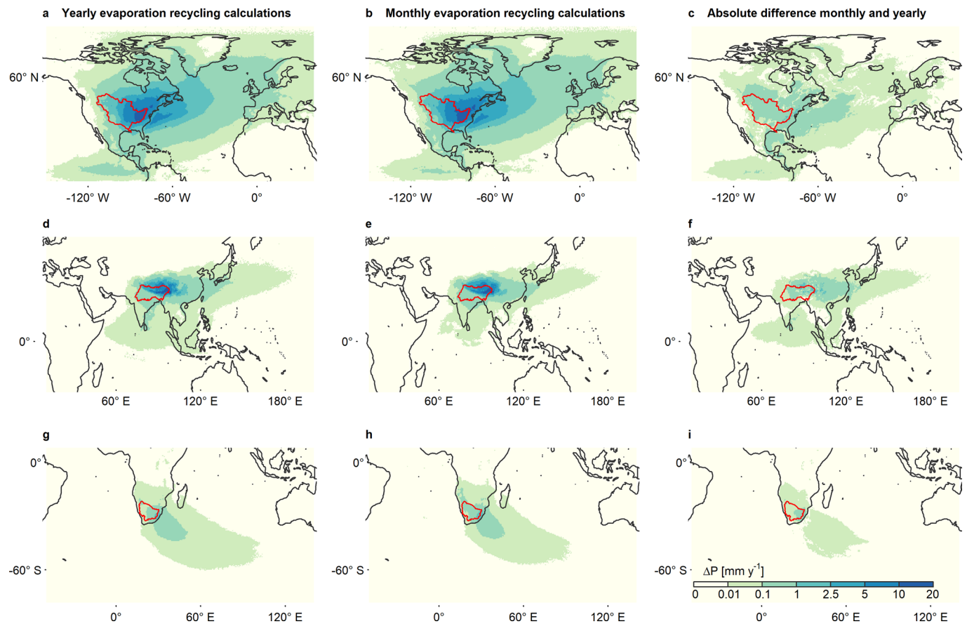
Extended Data Fig. 2 | Difference between yearly and monthly calculation of evaporation recycling from three river basins. In our study, we present the results based on a yearly calculation of evaporation recycling. This figure displays the difference between the applied yearly calculation and a monthly calculation of evaporation recycling. For the yearly calculation, the monthly evaporation recycling from the UTrack dataset is aggregated to yearly evaporation recycling. For the monthly calculation, the increase in evaporation (from Budyko) is disaggregated over twelve months, relative to the local monthly evaporation from the ERA5-reanalysis product 58 . Both the yearly and the monthly calculation in this figure display the yearly aggregated evaporation recycling. The figures display the increase in precipitation following a tree-restoration induced increase in evaporation from three different river basins: (a-c) Mississippi basin, (d-f) Ganges-Brahmaputra basin, and (g-i) Orange basin. (a, d, and g) display the yearly calculation, (b, e, and h) display the monthly calculation, and (c, f, and i) display the absolute difference between the monthly and yearly calculation.
