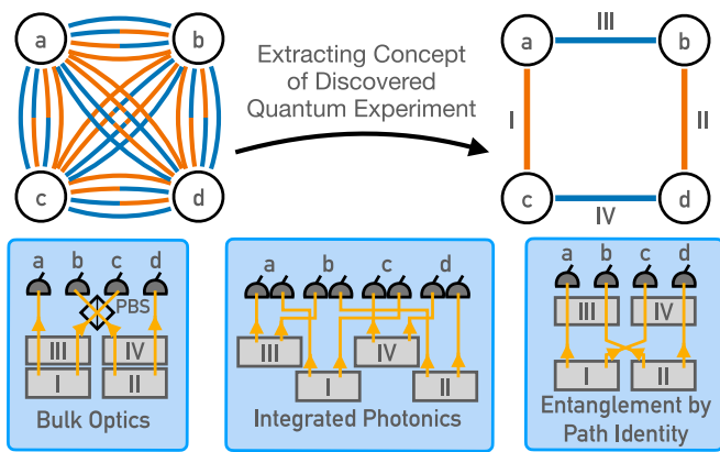
FIG. 6. Discovery of Quantum Experiments. Quantum optics experiments can be represented by colored graphs. Using the most general, complete graph as a starting representation, the AI’s goal is to extract the conceptual core of the solution, which can then be understood by human scientists. The solution can then be translated to numerous different experimental configurations [101].
