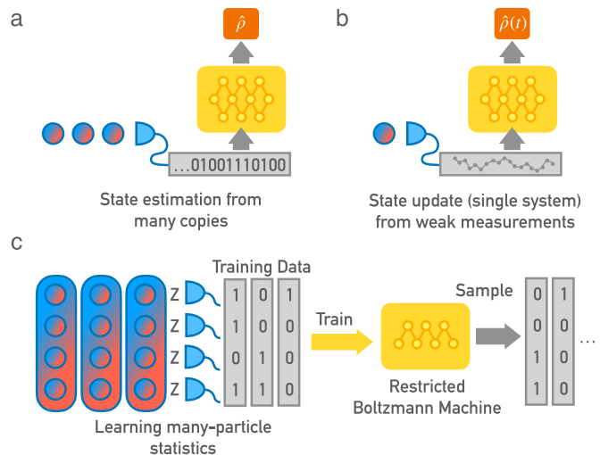
FIG. 3. State Estimation via Neural Networks. (a) Measurements on many identical copies of a quantum state can be processed to produce an estimate of the quantum state. (b) A continuous weak measurement on a single quantum system can be used to update the estimated state. Both in (a) and (b), a single network is trained to estimate arbitrary states correctly. (c) One can also train a network-based generative model to reproduce the statistics of a quantum state, i.e. to sample from the probability distribution. Training requires many identical copies that can be measured, so the statistics can be learned. Here, one network represents only a single quantum state. It can be extended to handle measurements in arbitrary bases.
