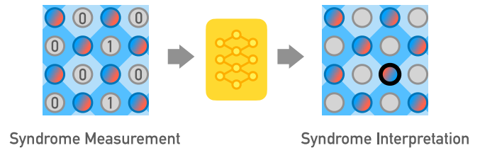
FIG. 8. Quantum Error Correction. Syndrome interpretation in a surface code as a task that a neural network can be trained to perform.
