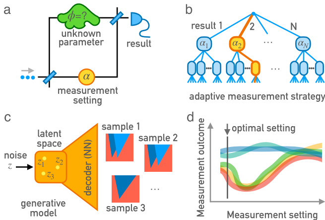
FIG. 4. Machine Learning for Parameter Estimation in Quantum Devices. (a) A typical scenario, with the measurement result statistics depending both on some tuneable measurement setting and the unknown parameter(s), here represented as phase shifts in a Mach-Zehnder setup. (b) An adaptive measurement strategy can be illustrated as a tree, with branches on each level corresponding to different measurement outcomes. Depending on those outcomes, a certain next measurement setting (indicated as “ \alpha_j ”) needs to be selected. Finding the best strategy is a challenging task, as it corresponds to searching the space of all such trees. (c) Neural generative models can be used to randomly sample possible future measurement outcomes (here: 2D current-voltage maps as in [56]) that are compatible with previous measurement outcomes. This is helpful for selecting the optimal next measurement location. Different random locations in latent space result in different samples. (d) Measurement outcome vs. measurement setting for 5 possible underlying parameter values (different curves; measurement uncertainty indicated via thickness). We aim to maximize the information gain, i.e. choose the setting which best pinpoints the parameter (which is not equivalent to maximizing the uncertainty of the outcome).
