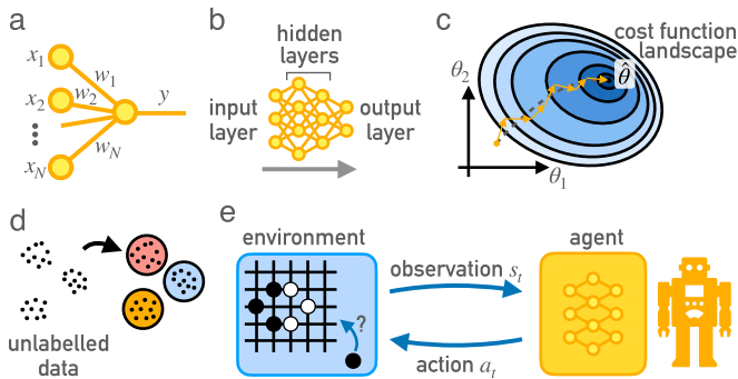
FIG. 2. Basics of Neural Networks and Machine Learning Techniques. (a) Operation of a single artificial neuron. (b) Structure of a neural network with dense layers. (c) Evolution of the network’s parameters \theta in the cost function landscape using stochastic gradient descent. For every step (orange arrows) the gradients of the averaged cost function with respect to \theta (gray dashed line) are approximated by the gradient averaged over a random batch. The parameters \hat{\theta} minimize the averaged cost function. (d) Classification of unlabelled data. (e) Reinforcement learning problem modelled as Markov decision process.
