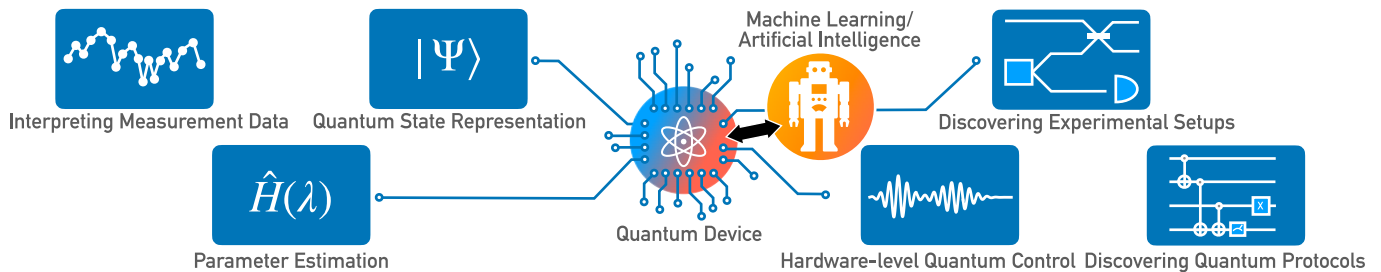
FIG. 1. Overview of tasks in the area of quantum technologies that machine learning and artificial intelligence can help solve better, as explained in this perspective article.
