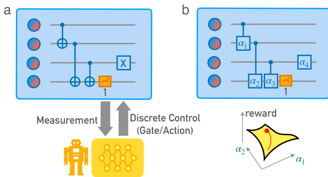
FIG. 7. Discovery of Quantum Circuits and Feedback Strategies with Discrete Gates. (a) A reinforcement-learning agent acts on a multi-qubit system by selecting gates, potentially conditioned on measurement outcomes, finding an optimized quantum circuit or quantum feedback strategy. (b) A fixed layout quantum circuit with adjustable parameters that can be optimized via gradient ascent to achieve some goal like state preparation or variational ground state search (possibly including feedback).
