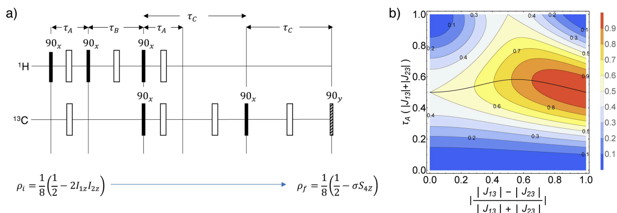
Figure 2. The pulse sequence used for polarization transfer is shown in panel a). The filled and open rectangles represent 90^\circ and 180^\circ pulses, respectively. The last dashed 90^\circ -pulse on the ^{13}\text{C} channel is used to store the heteronuclear magnetization along the applied magnetic field but dropped for direct observation of the HP signal. The phases of the 180^\circ pulses can be chosen at will along the transverse axes of the rotating radio-frequency frames, i.e. \pm x , \pm y . The sequence transfers PASADENA spin order 2I_{1z}I_{2z} into heteronuclear magnetization S_{4z} with efficiency \sigma , see Equation (2). Panel b) is the contour plot of the efficiency \sigma in function of the heteronuclear J -couplings J_{13} and J_{23} and of the time \tau_A at fixed \tau_B = 0.5/|J_{12}| and \tau_C = 0.5/|J_{34}| . The black line crossing the plot tracks the maximal efficiency path.
