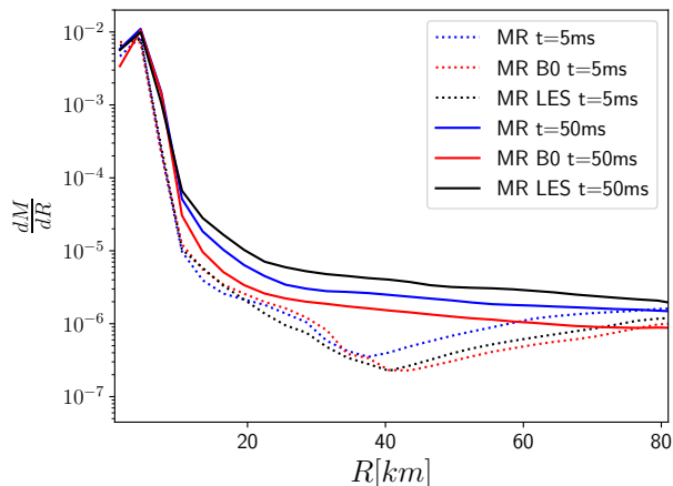
FIG. 15. Distribution of density in a solid angle near the axis. The mass contained in a solid angle of 15^\circ around the z -axis, for the medium-resolutions at t = 5 ms and t = 50 ms after the merger. This plot represents how the radial distribution of the mass increases with the magnetic field.
