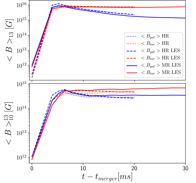
FIG. 6. Evolution of the average poloidal and toroidal magnetic field components. Contributions of the poloidal (blue) and toroidal (red) components to the magnetic field intensity, volume-averaged in the bulk (top) or in the envelope (bottom), for the medium resolution LES and the high-resolution simulations (linestyles).
