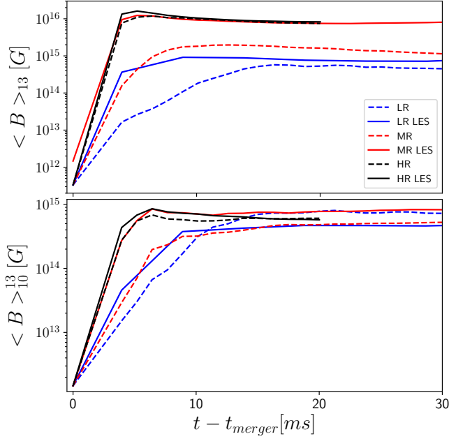
FIG. 5. Evolution of the average magnetic field. Volume-average of the magnetic field intensity either in the bulk (top) or in the envelope (bottom) of the remnant. These averages are calculated for all the resolutions (identified by colors), both for the LES (solid lines) and for the standard simulations (dashes). Clearly, the averages in the bulk calculated with LES converge to a well-defined value.
