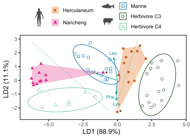
Figure 7. Linear discriminant analysis of compiled \delta^{13}\text{C}_{\text{essential amino acid}} data from human and faunal archeological bone collagen based on four essential amino acids (leucine, valine, phenylalanine, and lysine). The training data represent the three faunal groups and the predicted data of the two human sites. The median discriminant values of three faunal groups were significantly different (Pillai's trace = 1.39, F(4,66) = 37.5 , p < .001 ). The ellipses represent 95% prediction intervals of each faunal group, the convex hulls represent the outer group boundaries for each human site, and the arrows represent the relative weightings of the independent variables for creating the discriminant function. The symbols marked with asterisks denote outlier individuals. References: Terrestrial \text{C}_3 (Choy et al. 2010); marine, Herculeaneum (Rome, 79 CE; Soncin et al. 2021); and terrestrial \text{C}_4 , Nancheng (China, 2000–1600 BCE; Ma et al. 2021). See supplemental appendix S2 for sample information. Image: Silhouettes from PhyloPic ( http://phylopic.org ) under a Creative Commons license.
