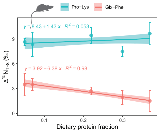
Figure 3. Regressions for pairs of amino acids between dietary protein content and the \delta^{15}\text{N} offset ( \Delta ) between trophic-source amino acids in mice muscle tissue. Higher dietary protein leads to smaller \Delta for the glutamic acid–phenylalanine but not the proline–lysine, pair indicating that the latter may provide more precise trophic position estimates in mammalian omnivores when the diet quality is unknown. The shading represents the 95% confidence interval of the regression lines for each trophic-source amino acid pair. Source: The data are from Whiteman and colleagues (2021). Image: Silhouette from PhyloPic ( http://phylopic.org ) under a Creative Commons license.
