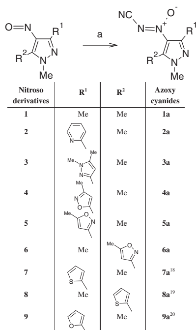
Scheme 1. Reagents and conditions: (a) \text{NH}_2\text{C}(\text{CN})\text{NH}_2\text{CN} , (diacetoxy)iodobenzene (IBA), dry \text{CH}_2\text{Cl}_2 , 30 °C.
