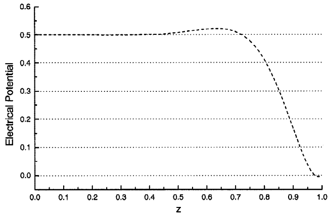
Fig. 4. Potential distribution, in the plane y = 0 , for a differentially heated duct, with T = z , M = 100 , and perfectly conducting walls. The velocity jet in the side layer is actually sustained by the potential gradient.
