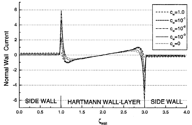
Fig. 18. Currents occurring normally at the walls in an internally heated duct, with Q = 1 , M = 1000 , and several values of c_w . As in the differentially heated duct, high currents flow in the side layers for the weakly conducting walls.
