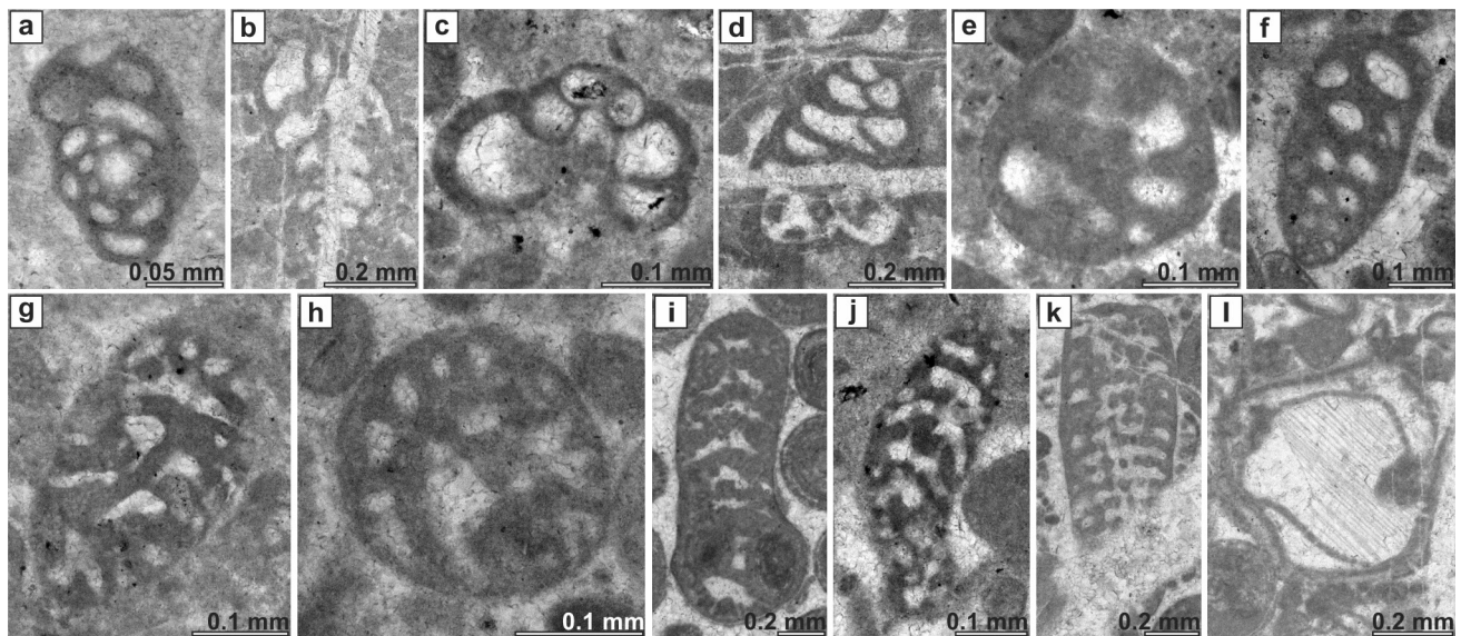
Fig. 8. Foraminifera from the Pliensbachian limestone in the antique quarry at Podpeč. a: Meandrovoluta asiagoensis Fugagnoli & Rettori. Thin section 1679. b: Siphovalvulina cf. variabilis Septfontaine. Thin section 1684. c: Siphovalvulina gibraltarensis BouDagher-Fadel, Rose, Bosence & Lord. Thin section 1679. d: Duotaxis metula Kristan. Thin section 1684. e: Pseudopfenderina butterlini (Brun). Transverse section. Thin section 1679. f: Pseudopfenderina butterlini (Brun). Oblique longitudinal section. Thin section 1679. g: Amijiella amiji (Henson). Oblique longitudinal section. Thin section 1679. h: Amijiella amiji (Henson). Oblique transverse section. Thin section 1679. i: Lituosepta sp. Longitudinal section. Thin section 1678. j: Lituosepta sp. Longitudinal section. Thin section 1679. k: ? Lituosepta sp. Longitudinal section. Thin section 1678. l: Thaumatoporella sp. Thin section 1684.
