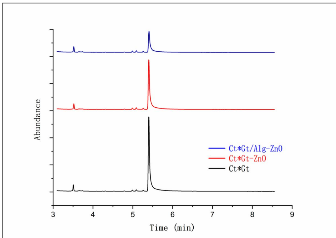
Figure S1: GC chromatogram for the removal of BPA by CS/GT, CS/GT /ZnO and CS/GT*m-Alg/ZnO beads.
