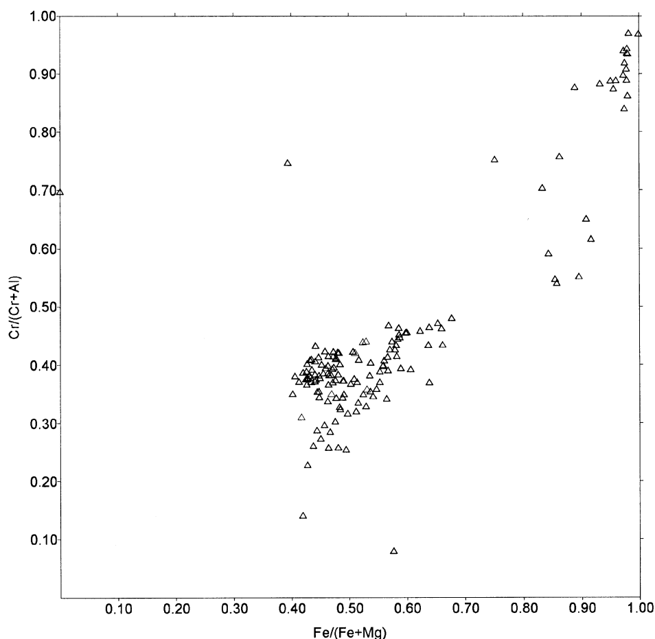
Fig. 4. Cr/(Cr + Al) – Fe/(Fe + Mg) plot of BAOC Cr-spinels. Points plotting above Cr/(Cr + Al) = 0.50 and above Fe/(Fe + Mg) = 0.70 represent altered spinels included in strongly metasomatised samples.
