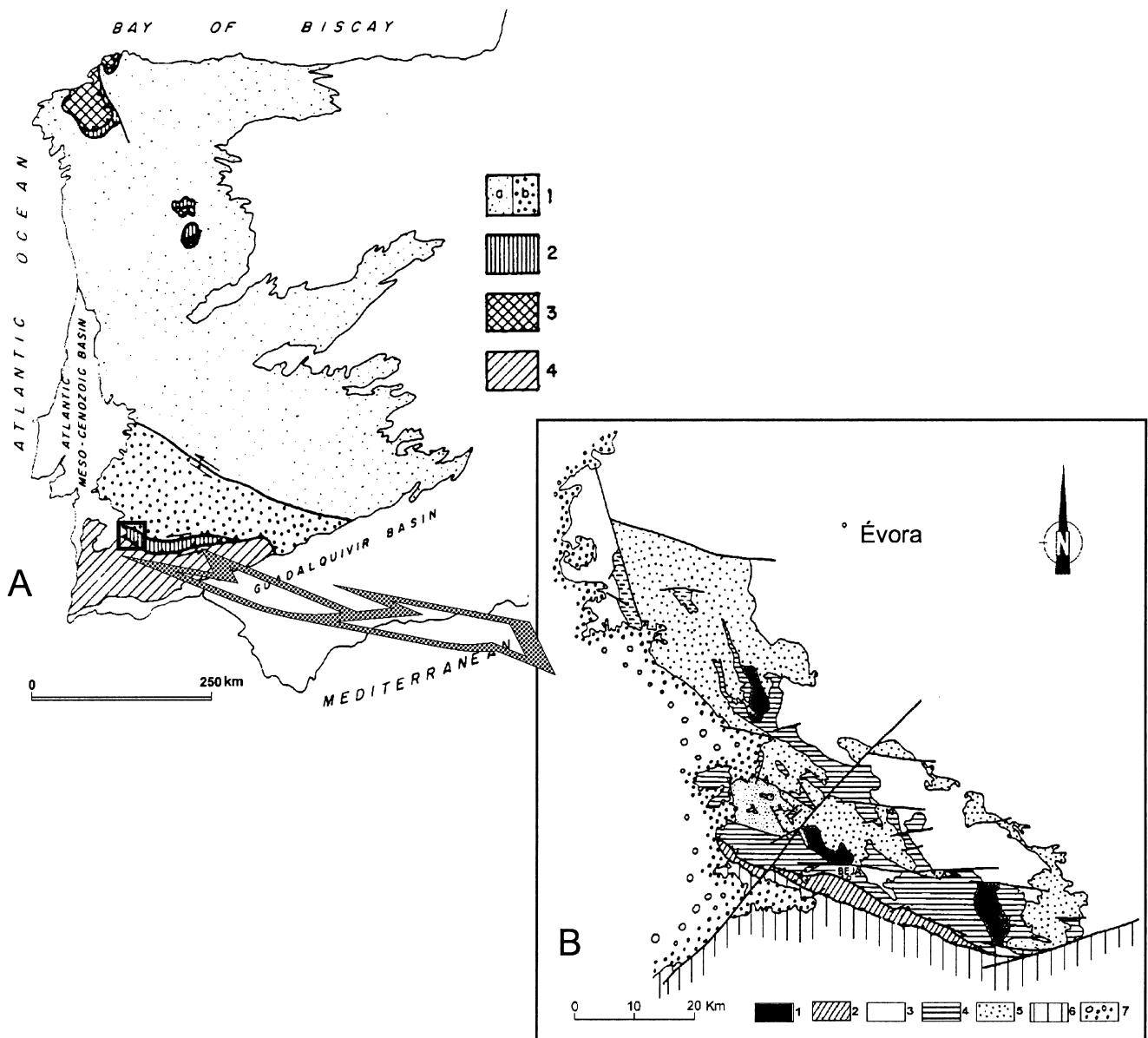
Fig. 1. A. Simplified tectonostratigraphic terrane map of the Iberian Massif (adapted from [28]): 1 – Proterozoic to Upper Paleozoic Iberian Autochthonous Terranes (a. Central Iberian Autochthon; b. Ossa-Morena Autochthon); 2 – Paleozoic Oceanic Terranes; 3 – NW Iberia Continental Allochthonous Terranes; 4 – South Portuguese Terrane. B – Simplified geological map of the Évora-Beja domain (adapted from [2]): 1 – Late Proterozoic to (Lower) Paleozoic imbricated units of the Ossa-Morena Zone; 2 – Mafic and ultramafic rocks of the Beja-Acebuches Ophiolite Complex; 3 – Paleozoic autochthonous rocks of Ossa-Morena Zone; 4 – Mafic and intermediate plutonic rocks of the Beja Igneous Complex; 5 – Acid plutonic and subvolcanic rocks of the Beja Igneous Complex; 6 – Pulo do Lobo metasedimentary group; 7 – Cenozoic sedimentary deposits.
