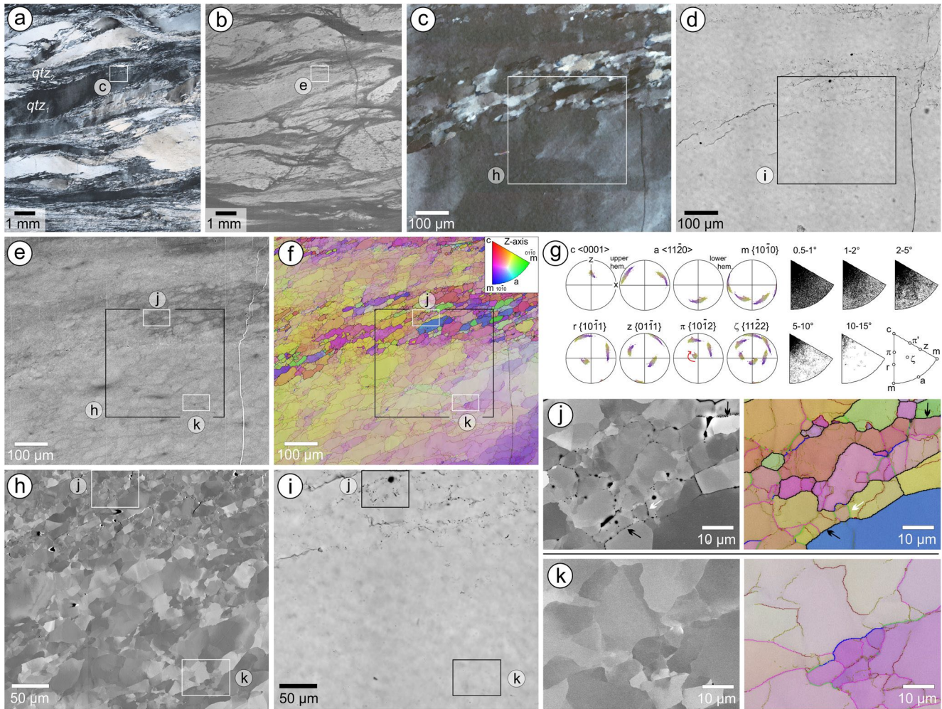
Figure 8. Site 2, quartz clast within (ultra)mylonitic matrix as marked in Figure 4e. (a) SEM-CL image with Ti-in-qtz data. SIMS analysis spots (c. 15 \mu\text{m} ) are color with respect to [Ti] – key is given. (b and c) Optical microphotographs (XPL, PL). Note, density of fluid-related GB pores in (c) corresponds with CL variation in (a). Black line in (a–c) indicates GB of quartz clast. (d) EBSD map (step size: 500 nm); transparent superposition of Euler and band contrast map. (a–d) Within the porphyroclast a localized cluster of fluid-related GB pores (b, c) associates with darker CL shades (a) and relates to an intracrystalline zone of recrystallized grains (d) (black arrows). (e) Orientation data of clast domains are presented as pole figures and misorientation axis plots of LAB (IPF and PF) – see Figure 6c. (f) Enlarged EBSD area as marked in (d). C-axis pole figure of recrystallized grains at the tip of the microshear zone is given – see inset. For Key of LAB and HAB see Figure 5. (g) Optical microphotograph (PPL) of area as marked in (f). (h) SEM-CL image of same area as presented in (g). CL variation corresponds to density of fluid-related GB pores shown in (g). In (f–h) black arrows mark intracrystalline deformation zone traced by HAB. White arrows mark recrystallization zone below the clast. “x” marks the position of the tip of the dark CL feature. Note, in the EBSD map (f) the location of “x” is several tenths of micron away from the recrystallized tip of the microshear zone and is located on the HAB between the upper and lower limb where no new recrystallized grains are developed. Oblique features in (g and h) are deformation lamellae.
