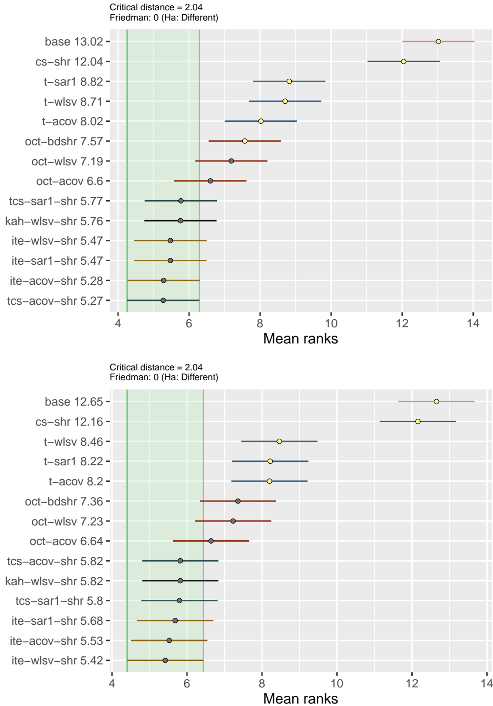
Figure A.13: Nemenyi test results at 5% significance level for all 95 series. The reconciliation procedures are sorted vertically according to the MAE mean rank for one-to-two-step-ahead (top) six-months forecasts and one-step-ahead twelve-months forecasts (bottom).
