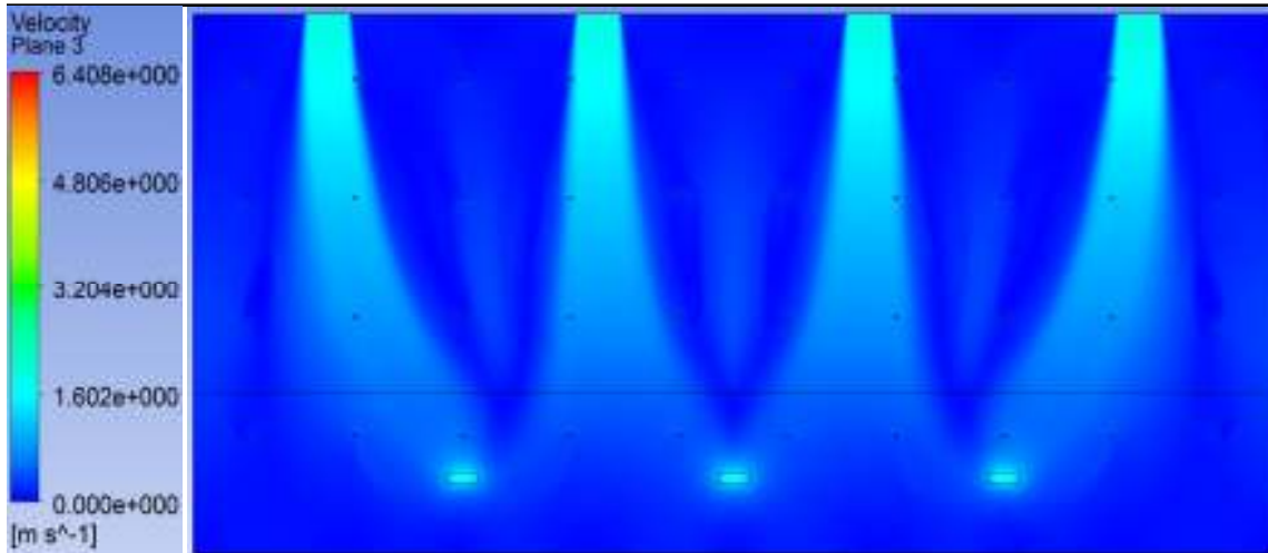
Figure 9-8 Configuration#1. Air velocity field inside the underfloor plenum for the 100% of peak load.
