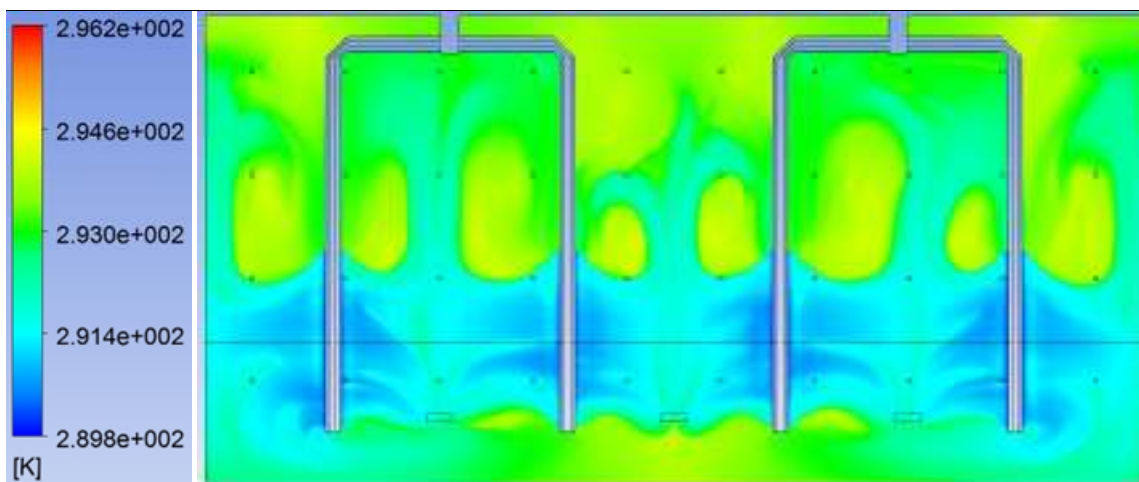
Figure 9-31 New model: temperature field
