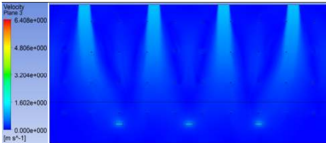
Figure 9-6 Configuration#1. Air velocity field inside the underfloor plenum for the 50% of peak load.
