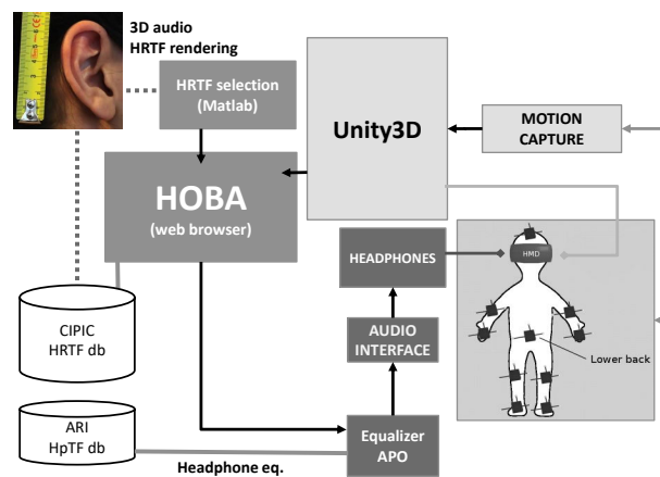
Figure 1. System overview.
