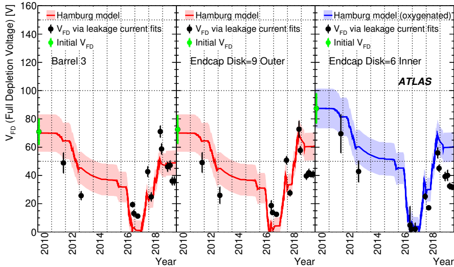
Figure 25. Evolution of V_{FD} estimated from the I-V curves. From left to right, results from barrel layer 3, outer ring of endcap disk 9 and inner ring of endcap disk 6 are shown. Green points show initial values of V_{FD} determined from C-V measurements. Predictions from the Hamburg model are shown by lines with model uncertainty bands for standard (red) and oxygenated (blue) silicon sensors.
