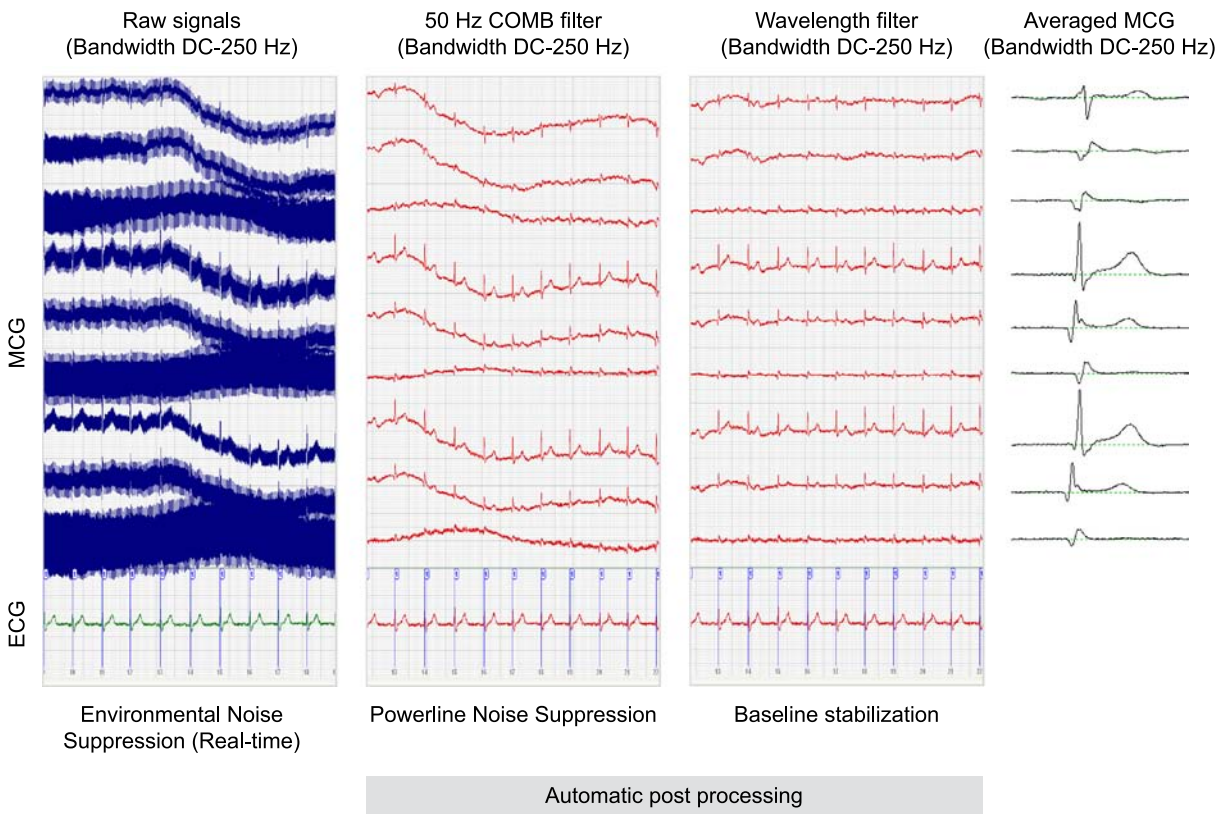
Fig. 2. Example of methods used to improve the S/N ratio of unshielded, in-hospital MCG recordings. Nine MCG channels and one (reference) ECG are shown. Real-time environmental noise suppression is provided by dedicated firmware. Digital filtering and signal averaging are automatic post-processing features. ECG = electrocardiogram; MCG = magnetocardiography; S/N = signal to noise.
