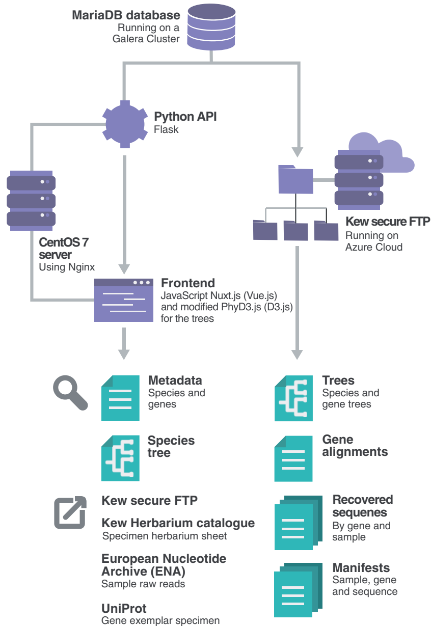
FIGURE 4. Data publication workflow. Implementation of the Kew Tree of Life Explorer data portal is illustrated. Arrows indicate data flow from internal repository to public interface. Infrastructural components are shown in upper half; publicly available information is shown in lower half. External links available from the portal are listed in the lower left.
