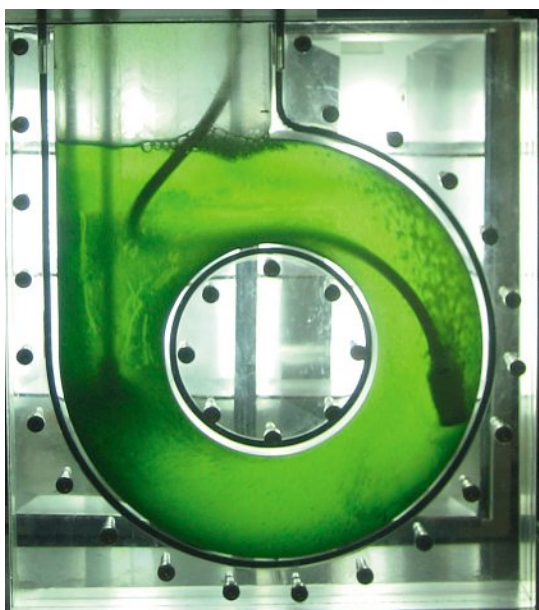
Fig. 3. Torus photobioreactor with micro algae cultivation.
