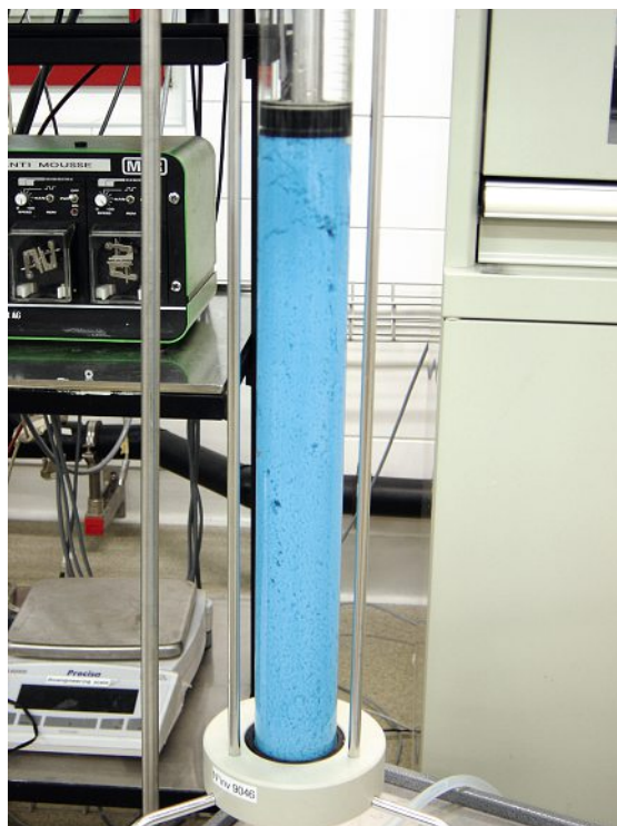
Fig. 4. Cu 2+ adsorption on a fixed bed of chitosan microbeads.
