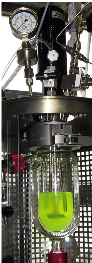
Fig. 1. Hydrogenation reactor.
