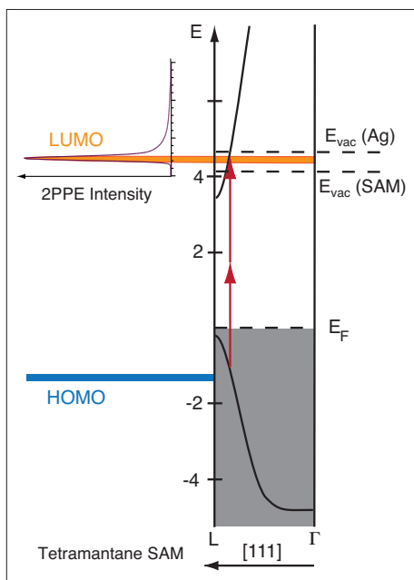
Fig. 4. Ag(111) substrate bandstructure and molecular orbitals in the [111]tetramantane-6-thiol SAM. The two-photon threshold transition into the LUMO (orange line) is indicated with red arrows. Adapted from ref. [42].
