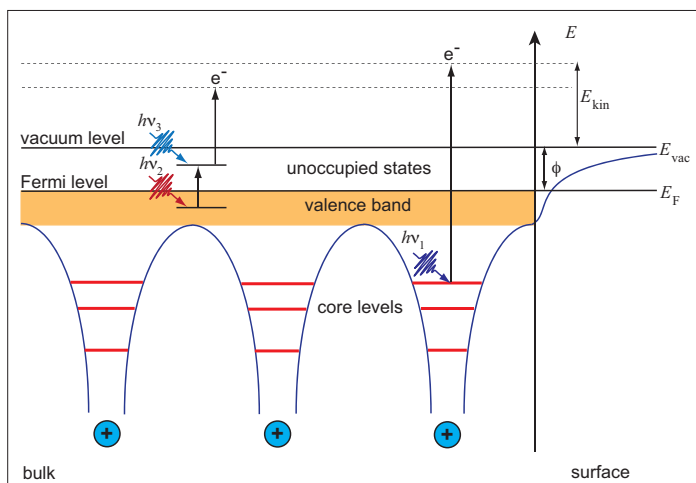
Fig. 1. Core and valence levels at a metal surface that can be probed by photoelectron spectroscopy. One X-ray photon ( h\nu_1 ) causes emission of a core electron. Two UV-VIS photons ( h\nu_2 and h\nu_3 ) cause emission of a valence band electron via an intermediate state above the Fermi level.
