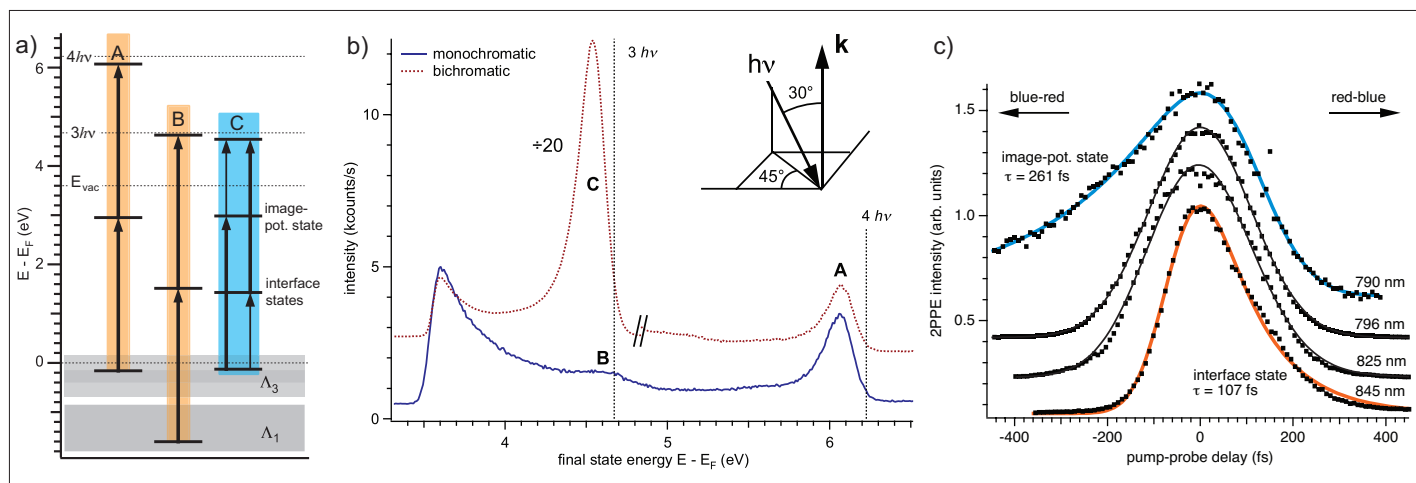
Fig. 2. (a) Energy level diagram deduced from experimental results. States observed in the 2PPE spectra are marked with horizontal lines. Monochromatic (orange) and bichromatic (blue) processes lead to different final states, short and long arrows indicate transitions at 796 and 398 nm, respectively. (b) 2PPE spectra of the h -BN/Ni(111) interface excited with 796 and 398 nm laser pulses. The monochromatic spectrum was taken using blue pulses only. (c) 2PPE intensity of feature C in the photoelectron spectrum as a function of pump-probe delay at different wavelengths. Adapted from ref. [37].
