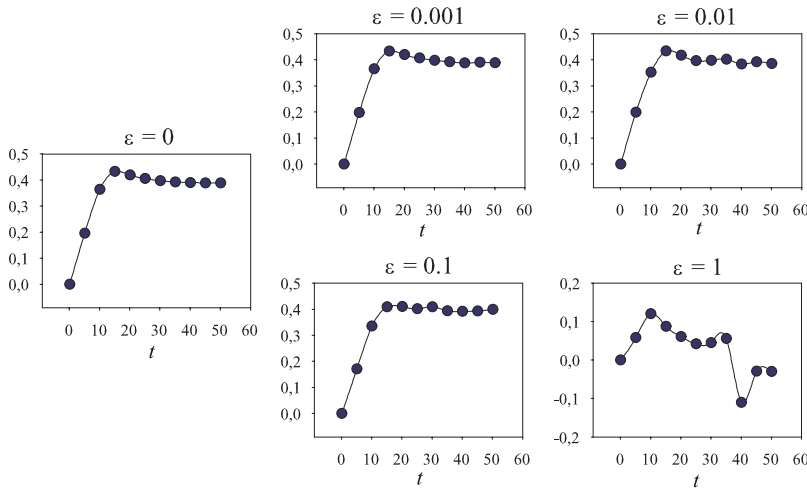
Fig. 5. Time evolution of the distance d_h(t) between the mean values of the fields distributions for different noise intensities, namely \epsilon = 0, 0.001, 0.01, 0.1, 1 .
