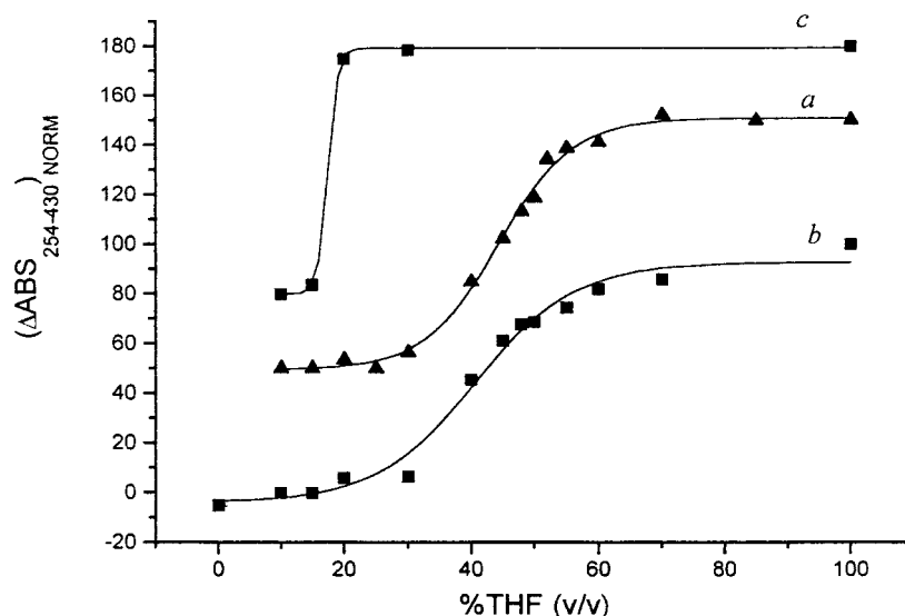
Figure 2. Aggregation (curves a and c) and dissociation (curve b) of AFE as a function of solvent composition in binary (THF–H 2 O, curves a and b) and ternary ([THF–(70%MeOH–30%H 2 O)], curve c) mixtures (v/v). Curves a and c have been translated along the ordinate axis, by 50 and 80 percentual units, respectively, for clarity.
