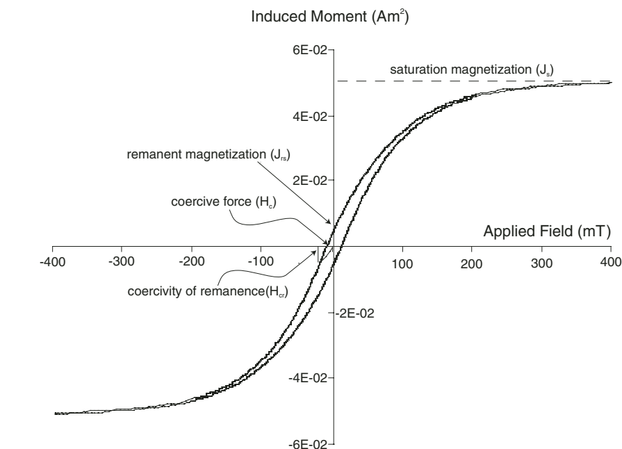
Figure 10. Hysteresis loop for sample Pieve d'Accinelli (PAC) 12.05, corrected for high field slope. The values for determining the size of a magnetite grain are J_s , J_r , H_c , and H_{cr} . H_{cr} represents the reverse field that, when applied and removed, cancels the J_{rs} value to make the magnetization of the sample zero.
