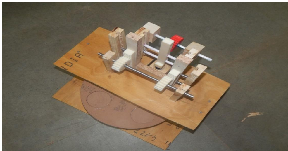
Fig 19: Final assembly
