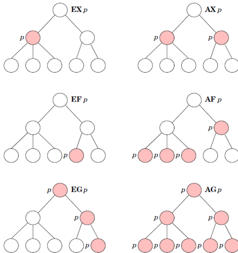
Figure 5.1: CTL Temporal Operators
