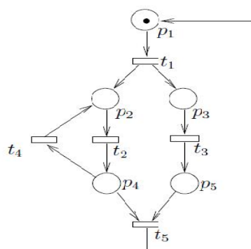
Figure 4.1: Stochastic Petri net
