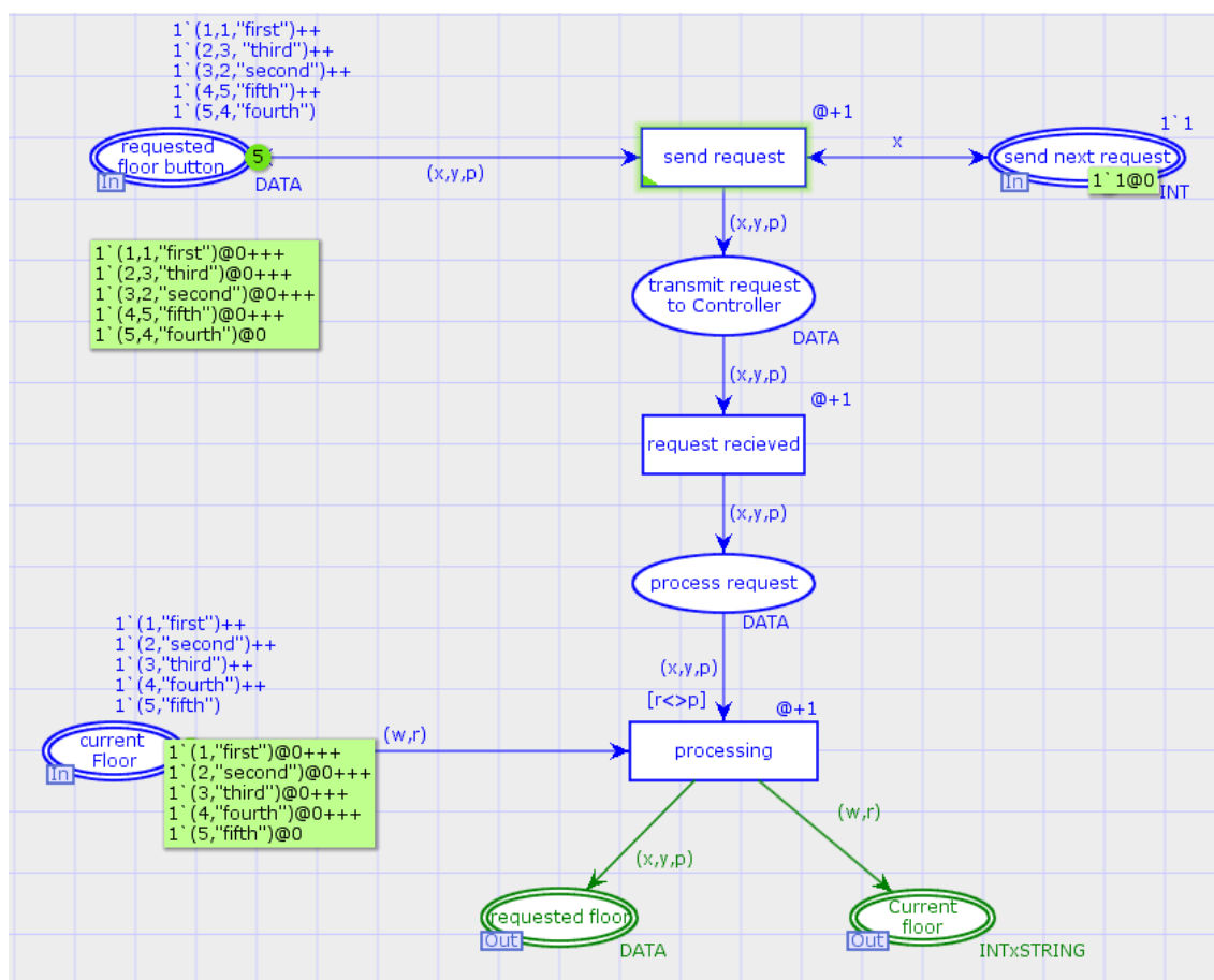
Figure 3.3: Processing of Request
