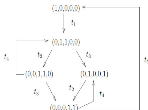
Figure 4.2: Reachability graph of SPN
