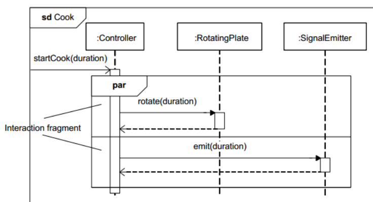
Figure 2.4: A sequence diagram with par interaction operator
