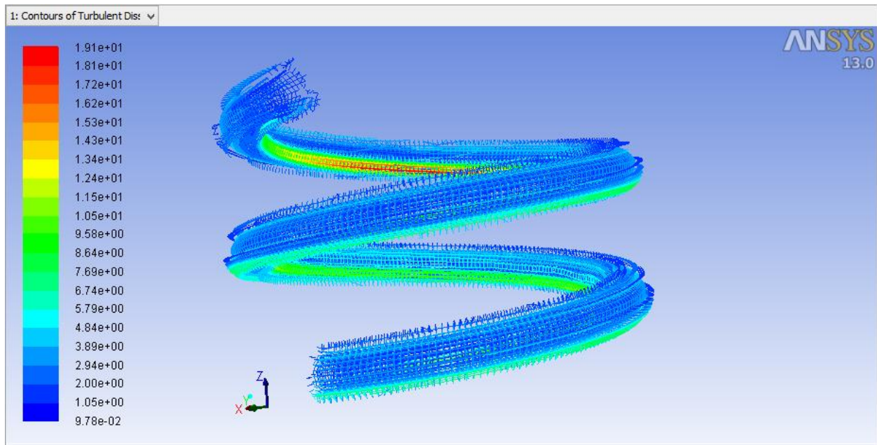
Contours of Turbulent Dissipation Rate (Epsilon) (m2/s3)
