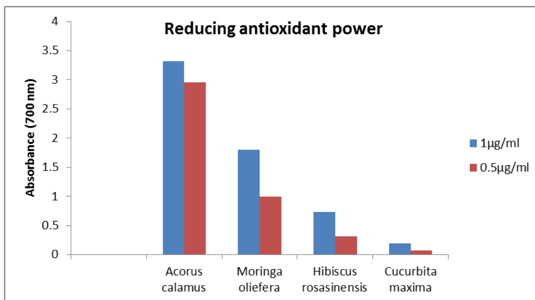
Fig 16: Reducing antioxidant power activity.
