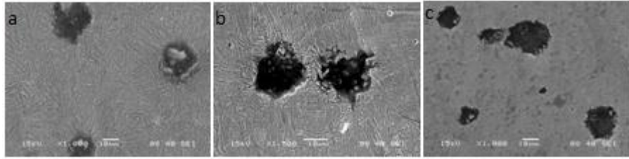
Fig.5.28.microstructure of the austempered ductile iron (without copper) austempered at (a) 250°C for ½ hour (b) 350°C for 1 hour (c) 300°C for 1 ½ hour.
