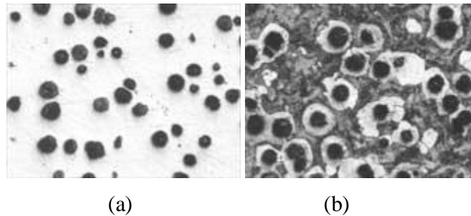
Fig 2.1. Microstructure of ductile iron (a) unetched (b) nital etched :100X [19].
