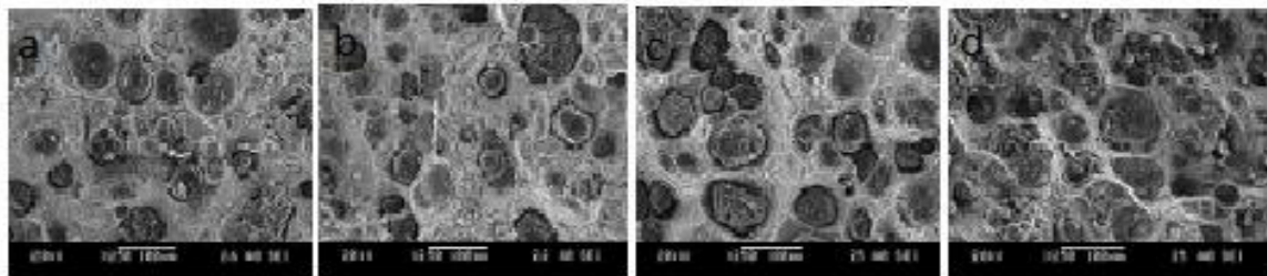
Fig.5.31. fracture surfaces of the austemered ductile (without copper) which austmpered at 250 0 C for (a) ½ hours (b) 1 hours, (c) 1 ½ hour and (d) 2 hours.
