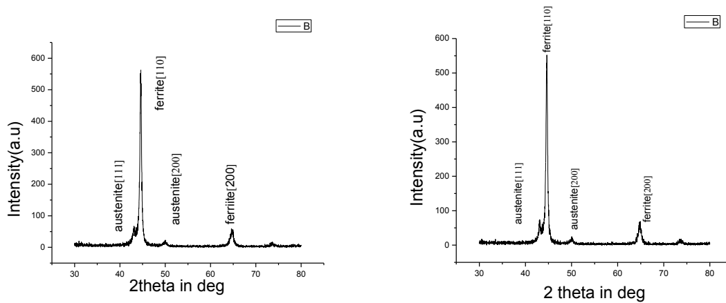
Fig.5.25. shows the XRD pattern of alloyed ductile iron austempered at 250 0 C for 1hour and 2 hours.
