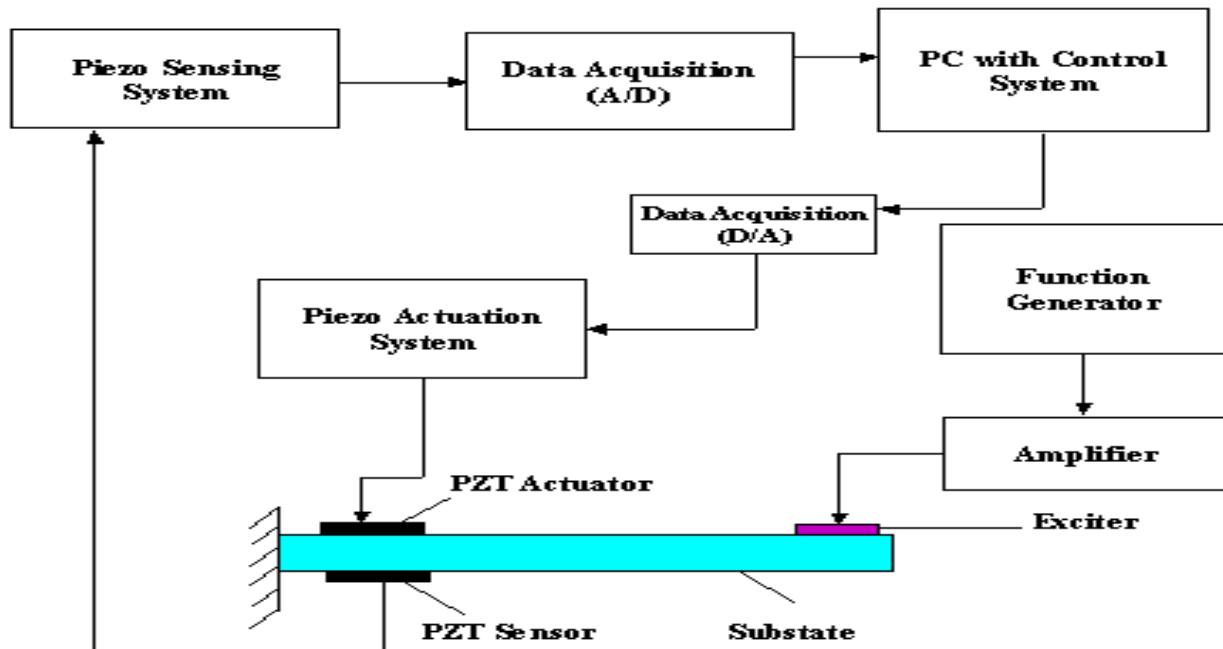
Fig. 7 Experimental setup [14]
