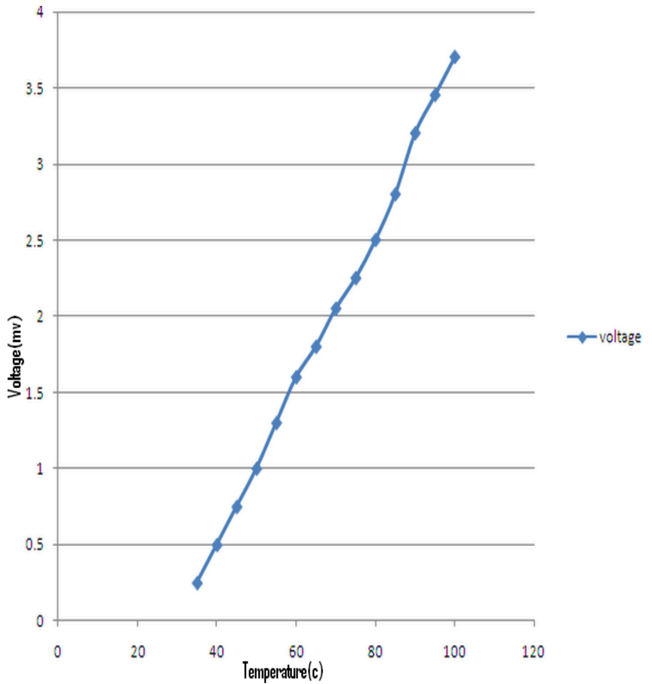
Temperature vs o/p voltage graph
