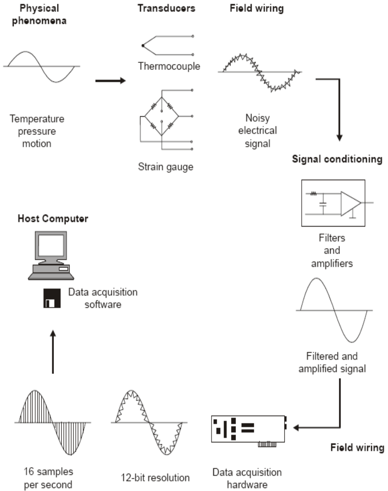
FUNCTIONAL DIAGRAM OF PC-BASED DATA ACQUISITION SYSTEM
