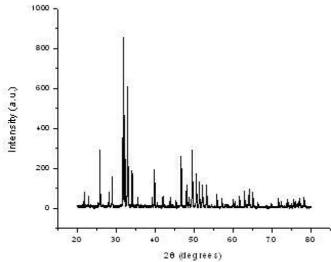
Fig. 4.3 XRD pattern of Hap at 1250 0 C
