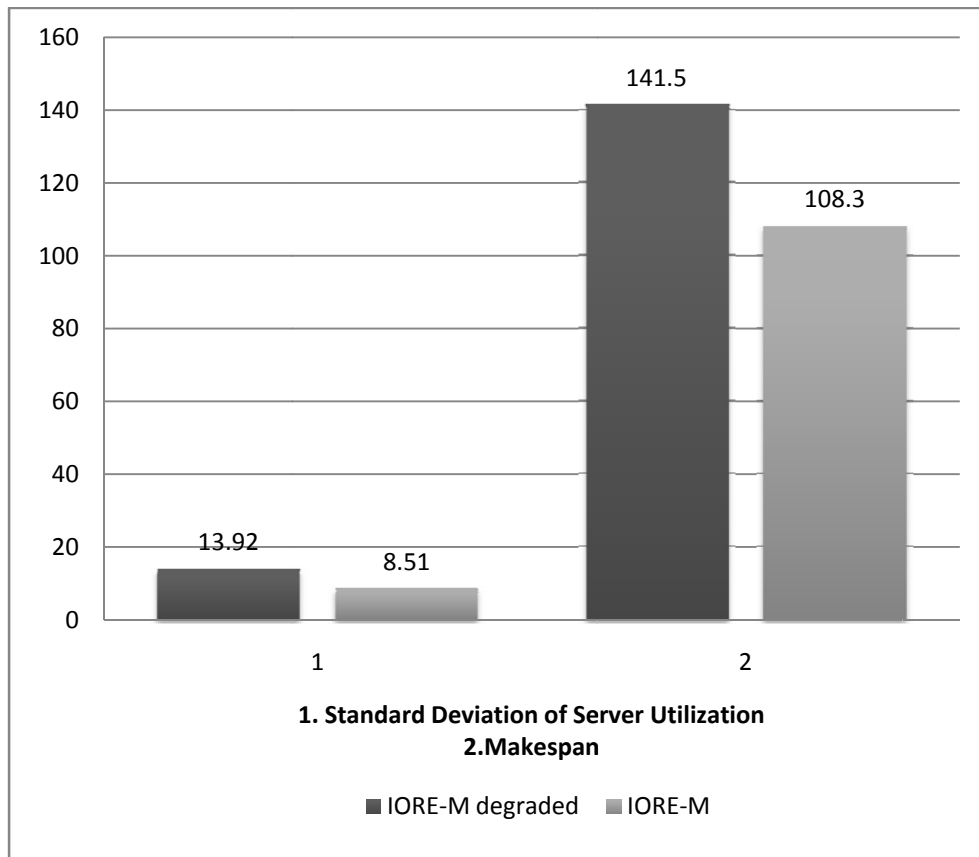
Figure 4.4 - Comparison of IORE-M and IORE-M degraded on system A
