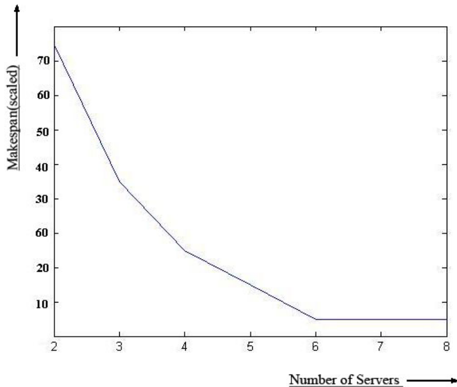
Figure 4.1 Determining no. of servers
