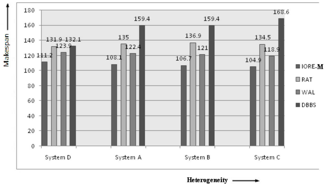
Figure 4.3 Comparison of scheduling makespan of different algorithms on different systems
