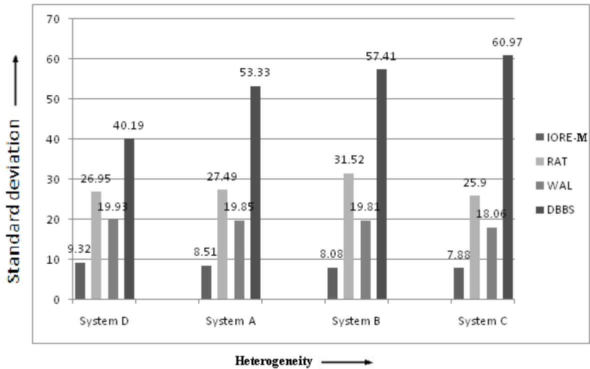
Figure 4.2: Comparison of standard deviation of server utilizations of different algorithms on different systems
